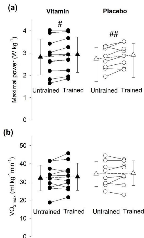
Figure 6. Three weeks of SIT increased power at exhaustion but not VO_{2max} . (a) Maximal power reached at task failure and (b) VO_{2max} during an incremental cycling exercise test prior to the first SIT session (Untrained) and two days after the last SIT session (Trained). Individuals were either treated with vitamins (black symbols; n = 10 ) or placebo (white symbols; n = 8 ). Data from each individual ( \bullet, \circ ) and mean data ( \pm SD; \blacktriangle, \triangle ). Two-way repeated measures ANOVA showed a significant training effect for maximal power in both groups ( \#, p < 0.05 ; \## p < 0.01 ); no training effect for VO_{2max} or difference between groups for any measurement was observed.
