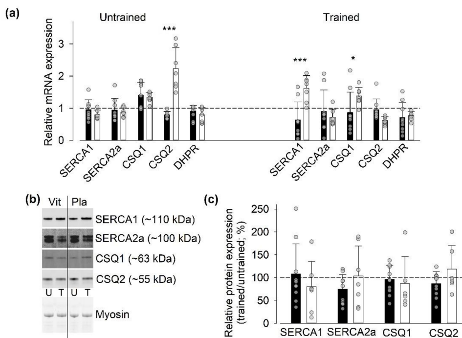
Figure 4. Limited SIT-induced changes in mRNA and protein expression of other SR Ca 2+ -handling proteins than RyR1. (a) Mean and individual data of the ratio of mRNA expression 1 h after to that before the first (Untrained) and last (Trained) SIT sessions in individuals treated with vitamins ( n = 9 ) or with placebo ( n = 7 ); dashed line indicates no difference between before and after exercise. Two-way repeated measures ANOVA showed a general group difference ( p < 0.01 ) in the untrained state. Difference between vitamins and placebo groups in relative mRNA expression of individual genes: * p < 0.05 , *** p < 0.001 . (b) Representative original Western blots from one individual treated with vitamins (Vit) and one treated with placebo (Pla). Biopsies taken before the first (untrained, U) and the last (trained, T) SIT session. Lower panels show stain-free loading controls. (c) Mean and individual data of the relative protein expression in biopsies obtained in the untrained and the trained state in individuals treated with vitamins ( n = 10 ) or with placebo ( n = 6-7 ). Data expressed as the ratio of the expression in the trained to that in the untrained state; dashed line indicate no difference between the two states. No significant differences between the untrained and the trained state or between vitamin and placebo-treated individuals were observed with two-way repeated measures ANOVA. Data are shown as mean \pm SD; vitamin group, black bars; placebo group, white bars.
