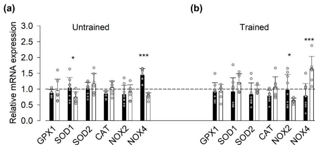
Figure 2. Vitamin-treatment-blunted sprint interval training (SIT)-induced changes in mRNA expression of genes encoding for reactive oxygen/nitrogen species (ROS)-related proteins in the trained state. Data (mean \pm SD) are expressed as the ratio of mRNA expression 1 h after to that before the first ((a), Untrained) and last ((b), Trained) SIT sessions. Vitamin group (black bars, n = 9 ); placebo group (white bars, n = 7 ); dashed line indicates no difference between before and after exercise. Data from each participant are shown as grey circles. Two-way repeated measures ANOVA showed a general group difference ( p < 0.05 ) in the trained state. Difference between vitamin and placebo groups in relative mRNA expression of individual genes: * p > 0.05 , *** p < 0.001 .
