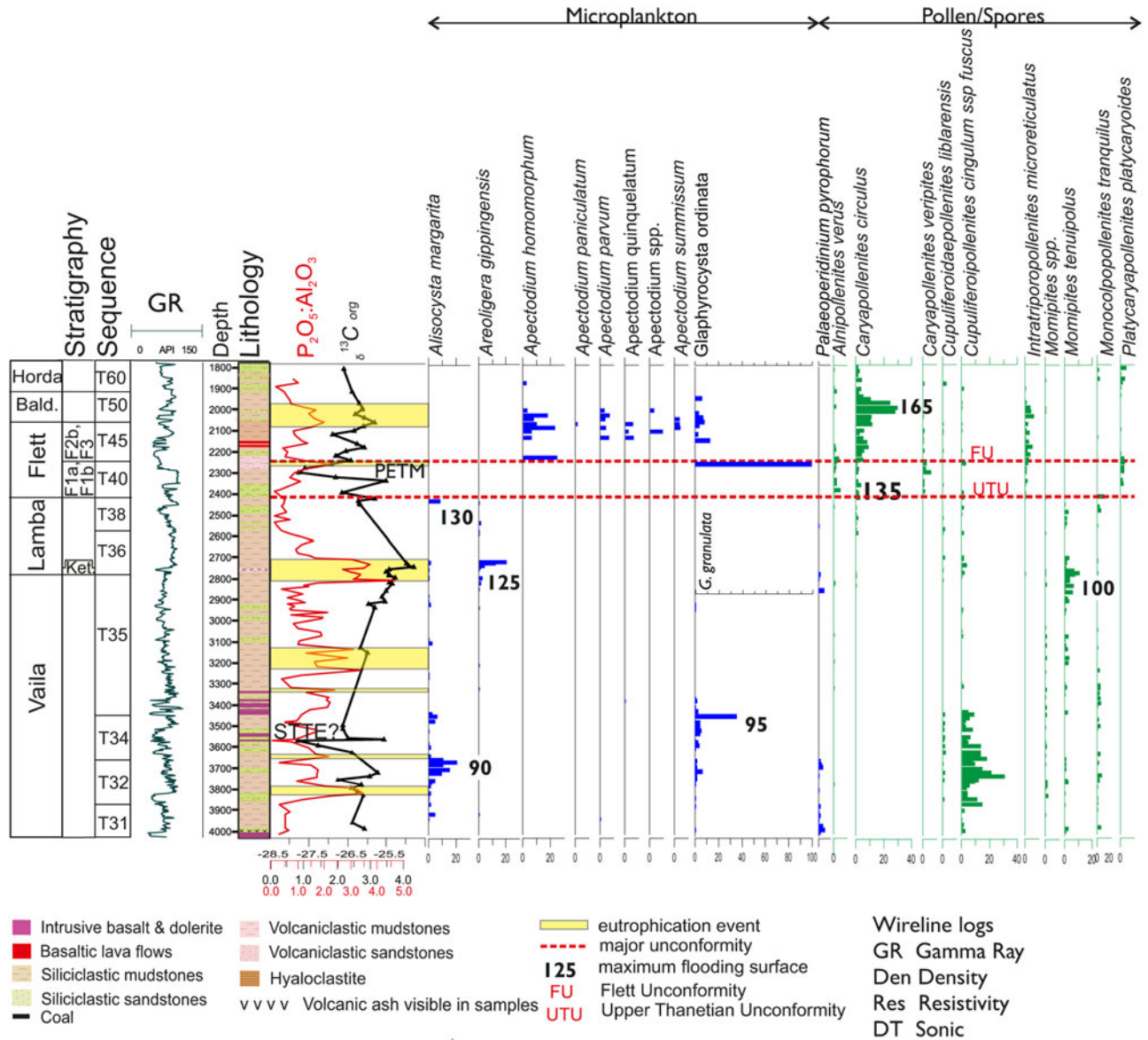
Figure 3 Well 6005/15-1: this well penetrated two thin syn-breakup basalt flows with an interbedded sedimentary unit, which yielded a palynoflora diagnostic of Sequence T45 (see Jolley 2009). The top of Sequence T40 is truncated by the Flett Unconformity, and Flett Formation strata below MFS 135 are missing, resting unconformably on the Lamba Formation (see Fig. 1 for lithostratigraphy used). Sequences T38 to T36 marine sedimentary rocks are marked by occurrences of Alisocysta margarita and Areoligera gippingensis in the Lamba Formation. At the base of Sequence T36, the Kettla Tuff Mb is recognised from its log signature and from the P_2O_5:Al_2O_3 plot, derived from FAAS of ditch cutting samples. This ratio highlights tephra-rich intervals in older Selandian sedimentary rocks, although these do not correspond directly to the cored interval of tuffaceous sediment (3508–3514 m; see Watson et al. 2017) because of ditch cuttings sample spacing. The \delta^{13}C_{org} record was derived from kerogen preparations. The upper part of the PETM record is missing at the Flett Unconformity. An older carbon isotope excursion is potentially a record of the STTE. All taxon palynomorph data displayed as percentages of total terrestrial or marine groups; only stratigraphically significant taxa are displayed. The standardised count of microplankton is plotted in this and subsequent figures to illustrate intervals of maximum marine influence. The key is common to all well stratigraphy figures and all wells are displayed in measured depths in metres (i.e., the depth in the well bore below a rig datum, usually the rotary table).
