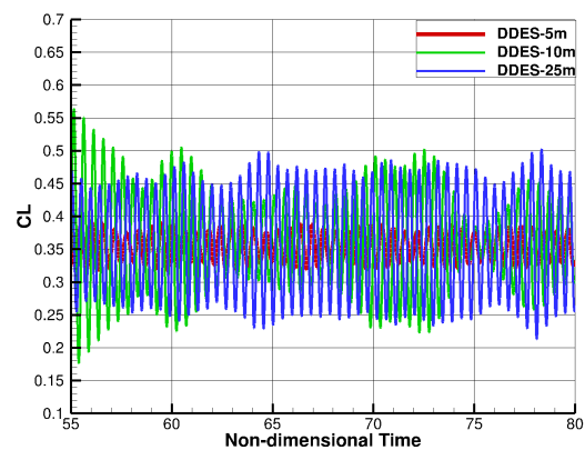
Figure 5: C_L time signal for the DDES simulations
