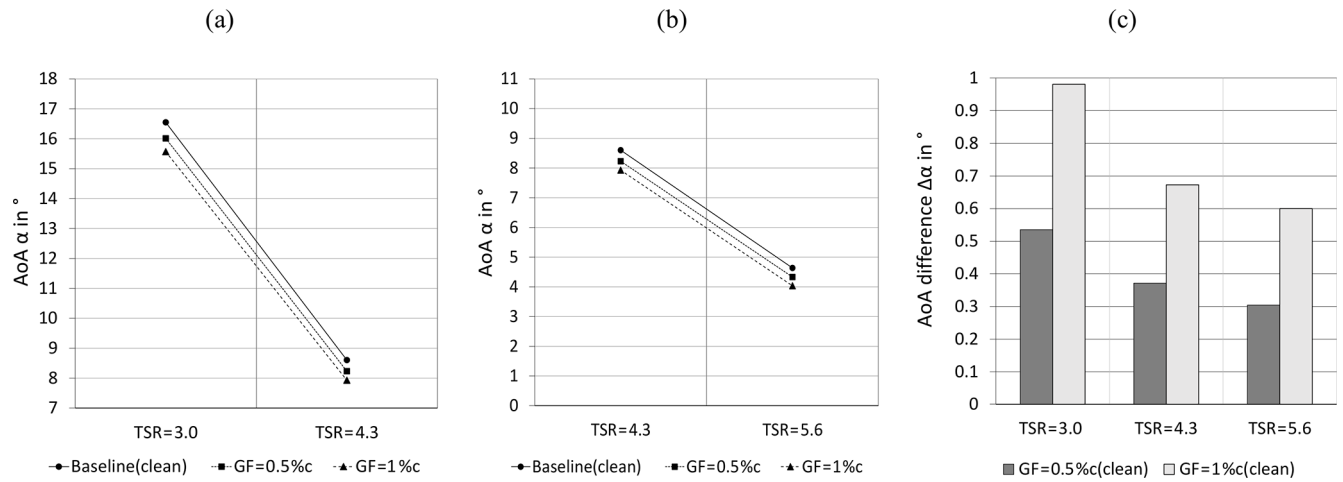
Figure A2. Angles of attack in the clean case at r = 0.56R and \varphi = 270^\circ . (a) Stall and rated conditions. (b) Rated and feather conditions. (c) AoA difference between Gurney flap configuration and the baseline.
