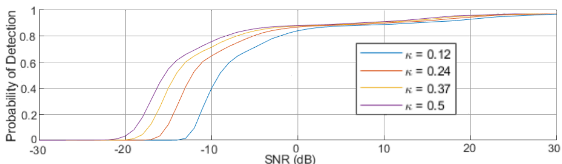
Figure 7. Detector performance for simulated satellite signal in an ISM environment.
