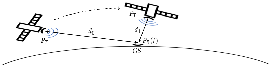
Figure 1. Communication link early in an overflight and close to the zenith.
