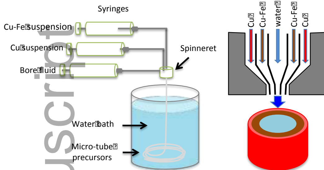
Figure 1. Schematics of the micro-tube preparation setup (left), the interior structure of the triple-orifice spinneret and the nascent micro-tube leaving the spinneret (right).
