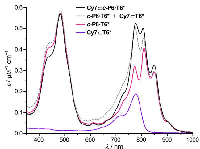
Figure 2. Absorption spectra of \text{Cy7@c-P6}\cdot\text{T6}^* (black), c -P6· \text{T6}^* (red), \text{Cy7@T6}^* (purple), and the addition of absorption spectra of c -P6· \text{T6}^* + \text{Cy7@T6}^* (gray dashed line), in \text{CH}_2\text{Cl}_2 at 25 °C.
