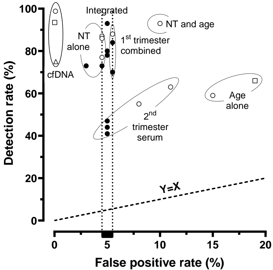
Figure 2. Twin Pregnancies: Receiver Operator Characteristic (ROC) Curve showing published point estimates of various Down syndrome serum/ultrasound screening combinations in the first trimester, second trimester and in both the first and second trimester. The horizontal axis displays the false positive rate while the vertical axis displays the corresponding Down syndrome detection (sensitivity) rate. Circles, squares and triangles indicate performance of identifying Down syndrome, trisomy 18 and trisomy 13, respectively. Open symbols show observed performance while the filled circles show modeled performance. Many of the data points are located at a 5% false positive rate (1-specificity), and the vertical dotted lines all indicate that same rate. This is done in order to avoid over-lapping test performance estimates. The straight dashed line ( Y=X ) indicates a 'useless' screening test.
