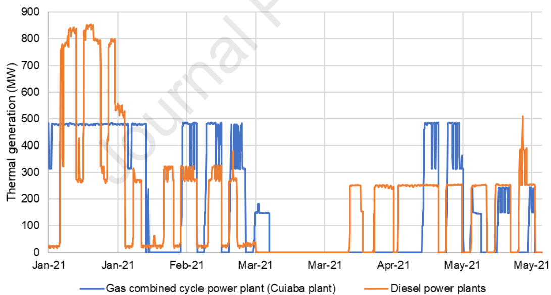
Figure 10: Thermal electric power generation with gas combined cycle and diesel power plant under the new operational scheme.
