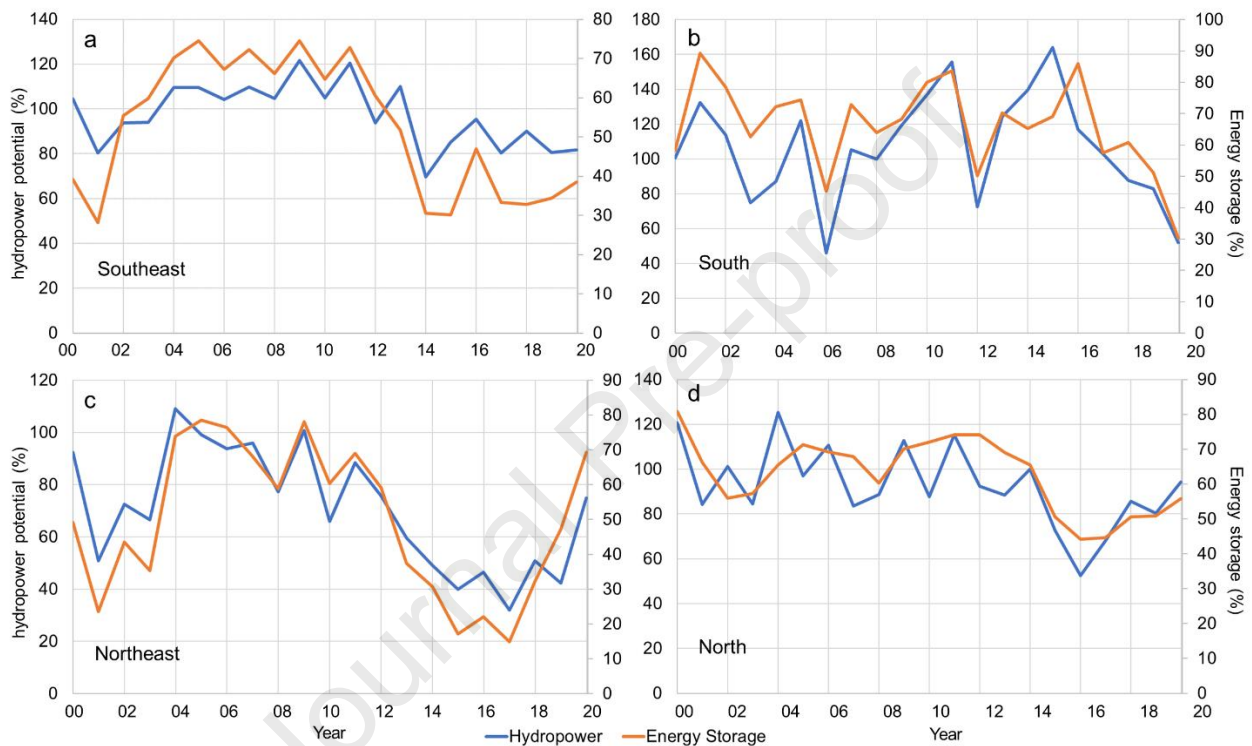
Figure 2: Comparison between the hydropower potential and the energy stored in the (a) Southeast, (b) South, (c) Northeast and (d) North regions of Brazil (years 2000 to 2020).
