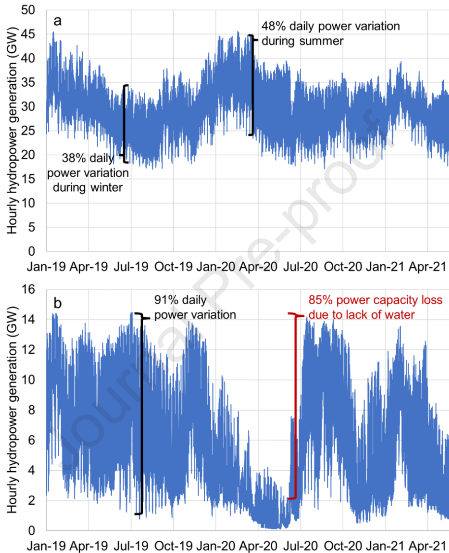
Figure 9: Power supply with hydropower in the (a) Southeast and (b) South region.
