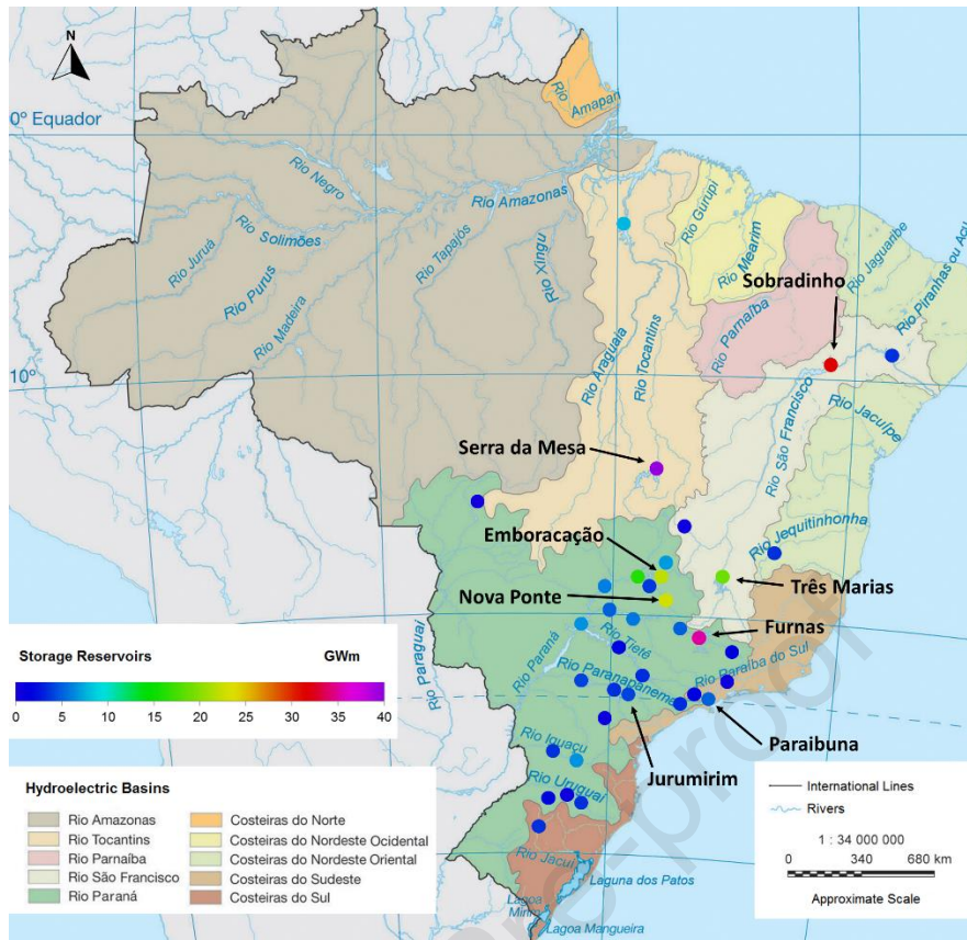
Figure 4: Main storage hydropower plants in Brazil and dams studied in this paper.
