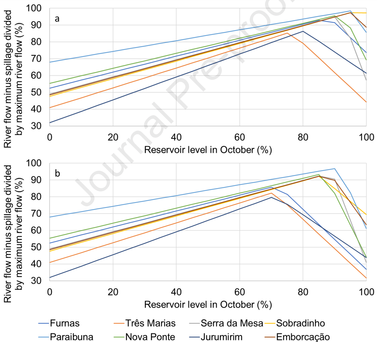
Figure 7: River flow minus spillage divided by maximum river flow (%), assuming (a) a generation capacity of 70% and (b) generation capacity of 50%.
