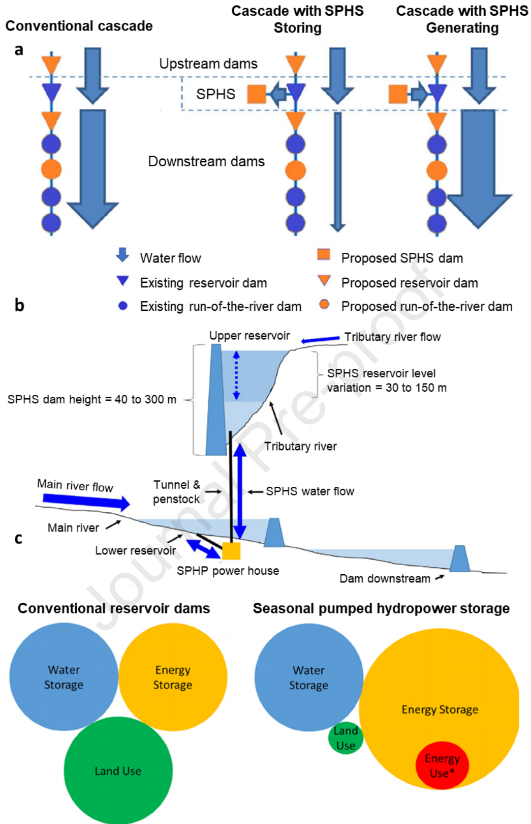
Figure 11: Seasonal pumped hydropower storage plants (a) represented in a cascade, (b) lateral view and (c) a comparison between water and energy storage, and land use [64] for conventional reservoir dams and SPHS plants.
