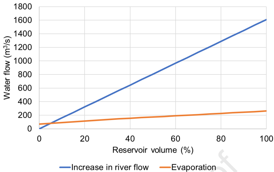
Figure 8: Comparison between the increase in river flow and evaporation with different reservoir levels.
