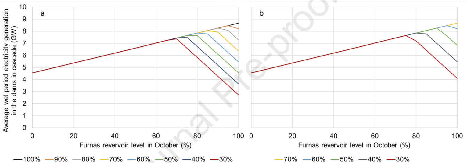
Figure 6: Average wet period electricity generation in the dams in cascade with different Furnas reservoir levels in October and different generation capacity factors in the dams in cascade (a) with existing installed capacity and (b) with 50% higher installed capacity.
