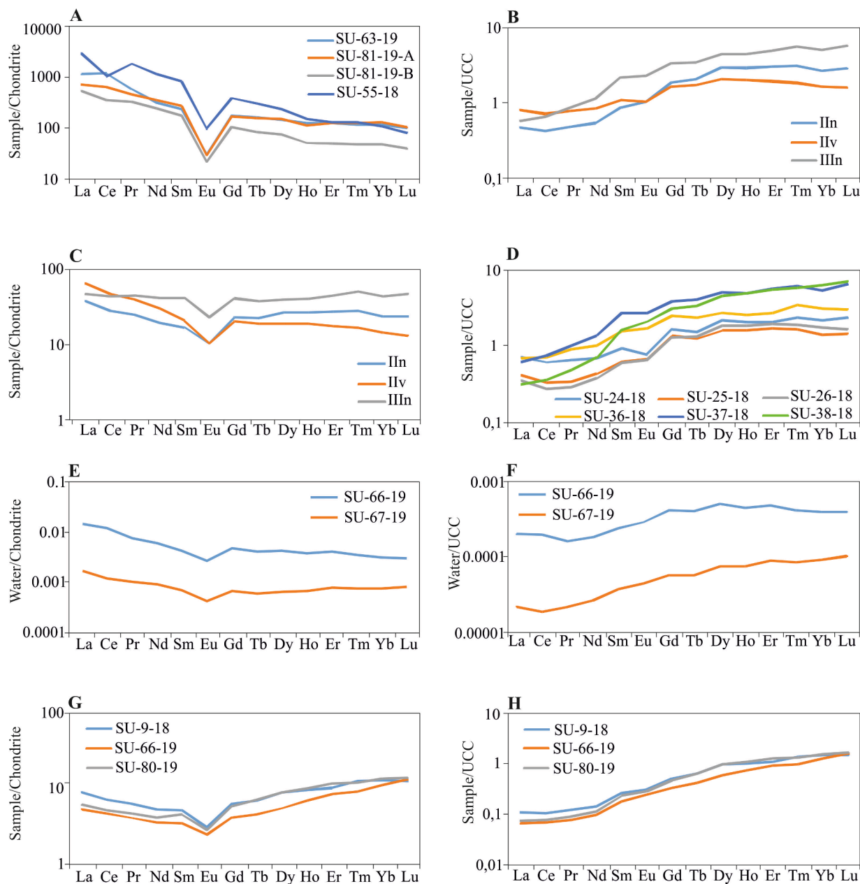
Fig. 8. Normalized graphs of the REE distribution in the granites of the basement (A), coal seams (B, C), coal seam IIII (D), drainage water (E, F) and carbonized wood (G, H) of the Spetsugli deposit. Note: * - normalized for chondrite according to (Taylor & McLennan, 1985); ** - normalized for the content in the upper continental crust according to (Taylor & McLennan, 1985).
