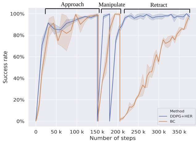
Fig. 5. Performance comparison of our training strategy using DDPG+HER and BC. Each experiment is executed independently three times with different seeds. Success is quantified as the percentage of successful grasp as a function of training steps.
