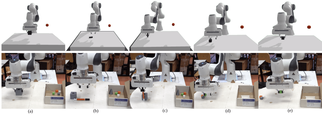
Fig. 3. Pick and place task (a) accomplished with end-to-end learning strategy with DDPG+HER and our LSE DDPG+HER. (b) failure with a thin cylindrical object for end-to-end strategy (c) success with a narrow cylindrical object for the agent trained with our LSE strategy. (d) failure with a small box object for the agent trained with end-to-end strategy. (e) success with a small box object for the agent trained with our LSE strategy.
