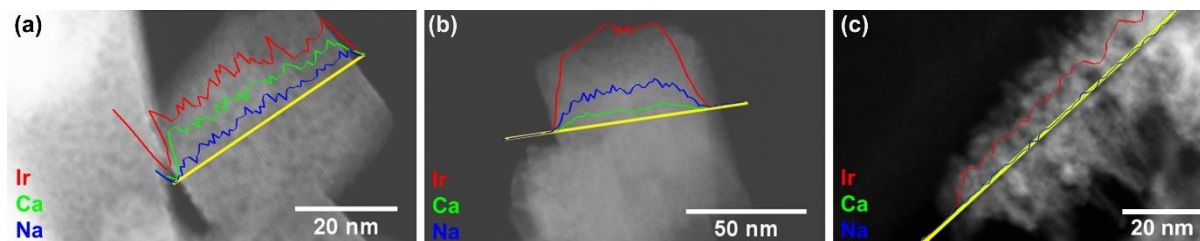
Figure 6: TEM and EDX linescans of (\text{Na,Ca})_{2-x}\text{Ir}_2\text{O}_6 \cdot n\text{H}_2\text{O} (a) as-made (b) acid-leached at 80 °C and (c) acid leached at 110 °C (18 M \text{H}_2\text{SO}_4 ). The yellow lines shows the scanned areas.
