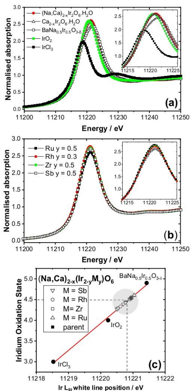
Figure 2: Ir L III -edge XANES spectroscopy: (a) XANES spectra of (Ca,Na) 2-x Ir 2 O 6 ·nH 2 O and Ca 2-x Ir 2 O 6 ·nH 2 O pyrochlores with reference materials where BaNa 0.5 Ir 0.5 O 3.8 was prepared according to the literature with \delta \approx 0.5 , 21 (b) XANES spectra of (Ca,Na) 2-x (Ir 2-y M y )O 6 ·nH 2 O materials and (c) analysis of the edge position to yield average oxidation state with the red line a linear fit to the reference materials and grey circle representing the scatter in edge positions of the substituted materials
