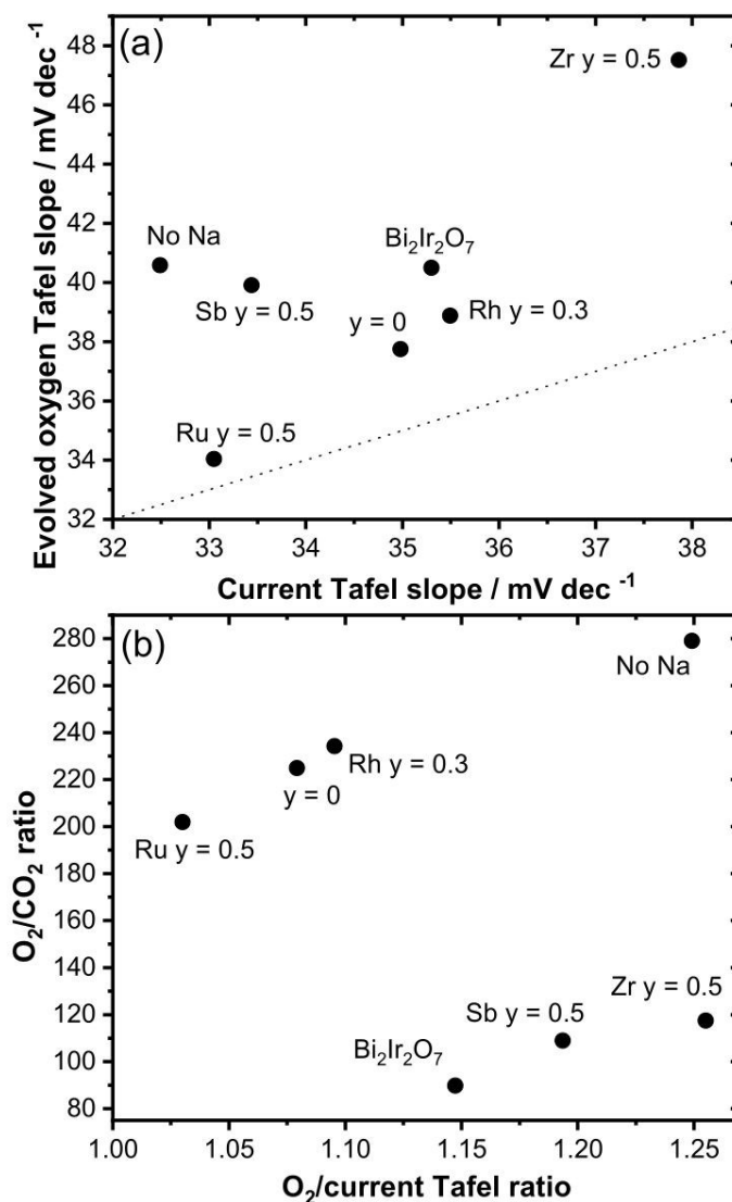
Figure 4: (a) Tafel slope values derived from analysis of current data and from evolved oxygen for (\text{Na,Ca})_{2-x}(\text{Ir}_{2-y}\text{M}_y)\text{O}_6 \cdot n\text{H}_2\text{O} ( \text{M} = \text{Sb, Zr, Ru, Rh} ) and \text{Ca}_{2-x}\text{Ir}_2\text{O}_6 \cdot n\text{H}_2\text{O} materials, with \text{Bi}_2\text{Ir}_2\text{O}_7 for comparison. The dotted line is the line where the current Tafel slope = evolved oxygen Tafel slope. (b) Plot of observed \text{O}_2/\text{CO}_2 ratios against the ratio of Tafel slopes determined by the two methods for the same materials.
