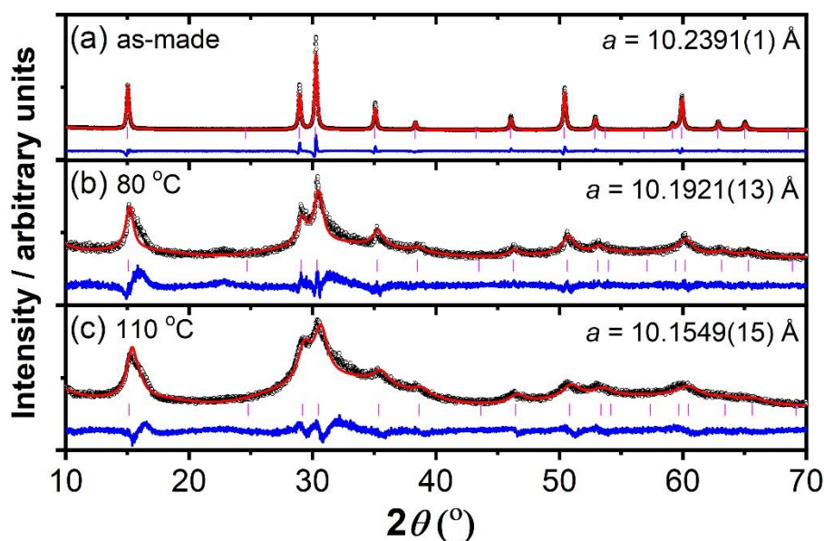
Figure 5: Powder XRD ( \text{Cu K } \alpha_{1/2} ) of (\text{Na,Ca})_{2-x}\text{Ir}_2\text{O}_6 \cdot n\text{H}_2\text{O} (a) as-made (b) acid-leached at 80 °C and (c) acid leached at 110 °C (18 M \text{H}_2\text{SO}_4 ). The points are the measured data, the red line the fitted profile, the blue line the difference curve and the pink ticks the positions of allowed Bragg peaks. The refined lattice parameters are given on each plot.
