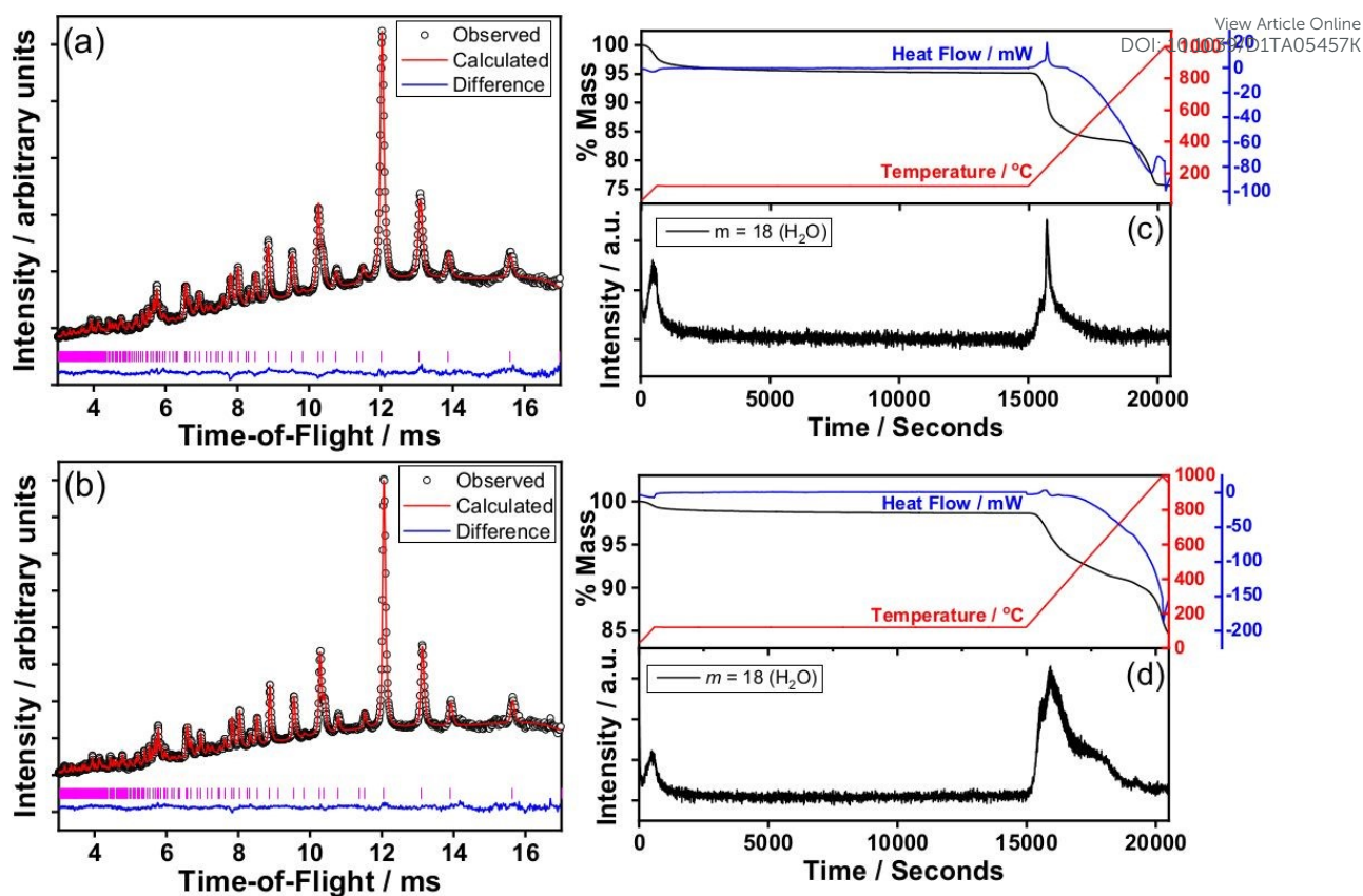
Figure 1: Characterisation data from iridate pyrochlores: (a) and (b) shows plots of the Rietveld refinement against neutron patterns (bank 5, GEM) of (\text{Ca,Na})_{2-x}\text{Ir}_2\text{O}_6 \cdot n\text{H}_2\text{O} and the sodium-free analogue \text{Ca}_{2-x}\text{Ir}_2\text{O}_6 \cdot n\text{H}_2\text{O} , respectively. Pink tick marks show the positions of allowed Bragg peaks (space group Fd\bar{3}m ; see Table 1 for refined structural parameters.) (c) and (d) show TGA-DSC-MS from (\text{Ca,Na})_{2-x}\text{Ir}_2\text{O}_6 \cdot n\text{H}_2\text{O} and \text{Ca}_{2-x}\text{Ir}_2\text{O}_6 \cdot n\text{H}_2\text{O} pyrochlores showing the presence of both surface and crystal water (see text for discussion).
