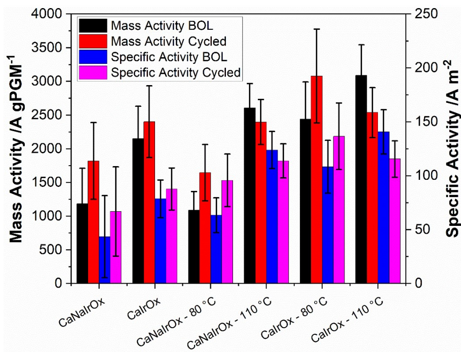
Figure 7: Electrocatalytic performance of pyrochlores (\text{Na,Ca})_{2-x}\text{Ir}_2\text{O}_6 \cdot n\text{H}_2\text{O} (denoted CaNaIrOx) and \text{Ca}_{2-x}\text{Ir}_2\text{O}_6 \cdot n\text{H}_2\text{O} (denoted CaIrOx) as-made and with acid treated, with the temperatures of acid-treatment noted. BOL = beginning of life.
