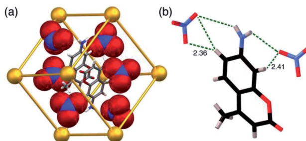
Fig. 3 Views of the crystal structure of H · MAC ·( \text{NO}_3 ). (a) A view showing the metal ions that define the cubic cage, the MAC guests, and the array of six nitrate anions around the surface (shown space-filling); (b) a view showing \text{CH}\cdots\text{O} and \text{NH}\cdots\text{O} interactions between a MAC guest and two of the surrounding nitrate anions.
