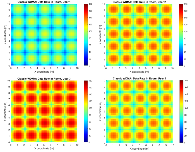
Figure 2: Achievable data rate distribution in a 10x10x3 m room for 4 users employing Classic WDMA without the contribution of the PS phenomenon. The assigned channel is fixed for each user.
