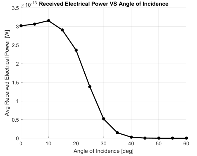
Figure 1: Average received electrical power vs angle of incidence. The received electrical power is averaged over four RGBA LEDs transmitting to four RGBA-filtered receivers. Due to the PS phenomenon, said power decreases substantially while increasing the AoI.
