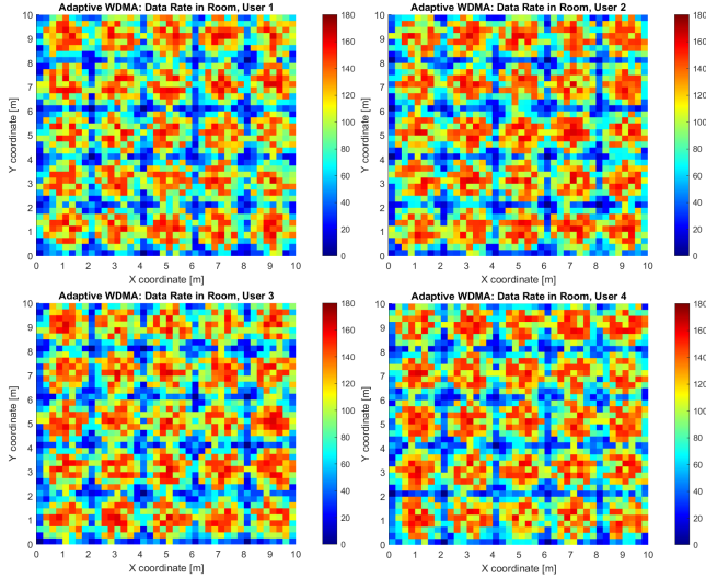
Figure 4: Achievable data rate distribution in a 10x10x3 m room for 4 users employing Adaptive WDMA including the contribution of the PS phenomenon. The assigned channel is determined for each user by maximising the aggregate SINR.
