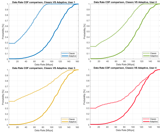
Figure 5: CDF of data rate comparison for 4 users employing Classic VS Adaptive WDMA. Each CDF is obtained over 10.000 iterations in which each user has a random position and orientation.
