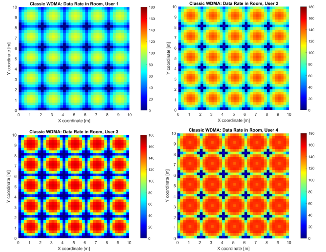
Figure 3: Achievable data rate distribution in a 10x10x3 m room for 4 users employing Classic WDMA including the contribution of the PS. The assigned channel is fixed for each user.
