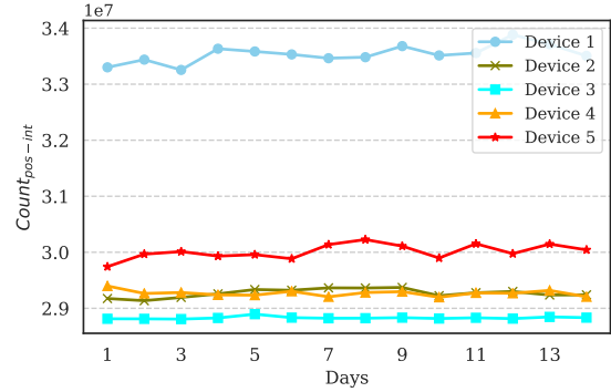
(d) Variation in daily averages of position count of internal oscillator - Count_{pos-int}
