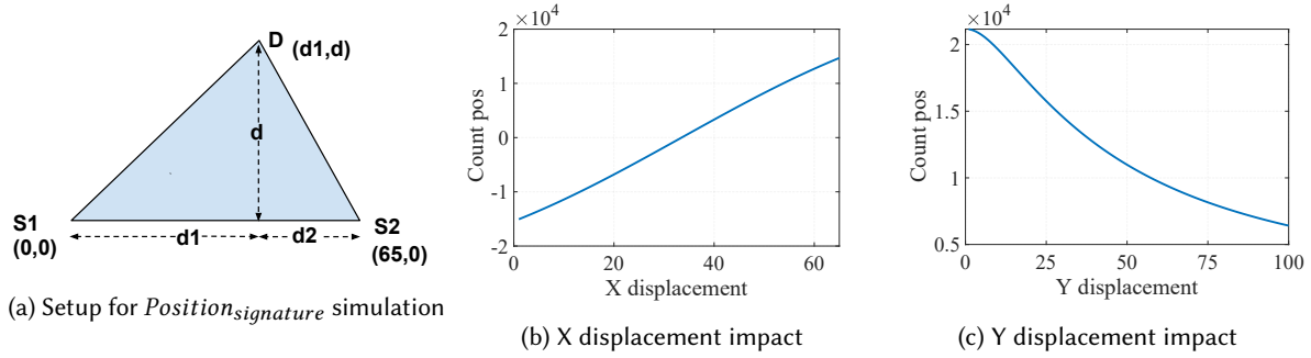
Fig. 6. Principle of Position_{signature} generation
