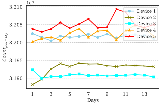
(c) Variation in daily averages of position count of crystal oscillator - Count_{pos-cry}
