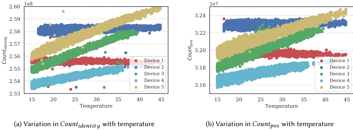
Fig. 14. Variation in Acoustic PUF with temperature
