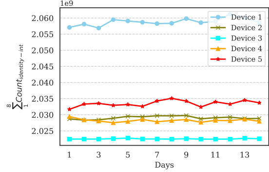
(b) Variation in daily averages of accumulated identity count of internal oscillator - Count_{identity-int}
