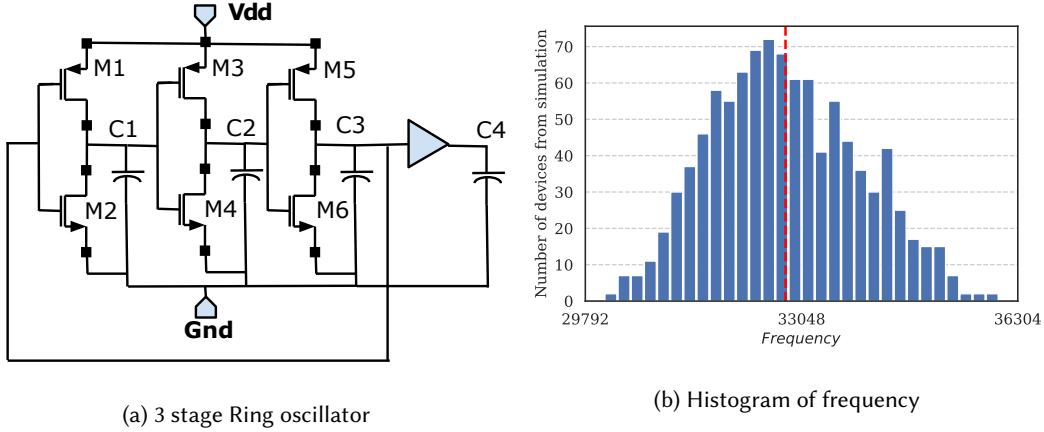
Fig. 5. Monte Carlo simulations for ring oscillator
