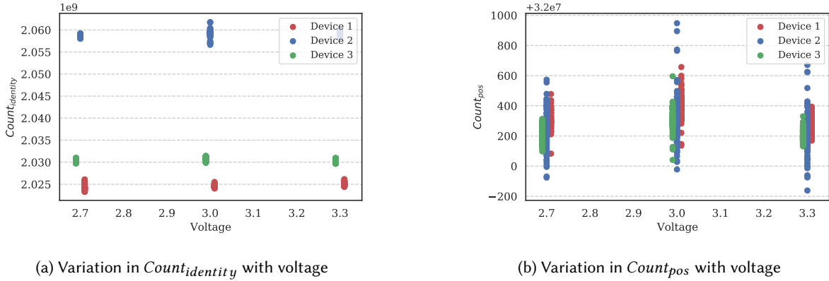
Fig. 15. Variation in Acoustic PUF with voltage
