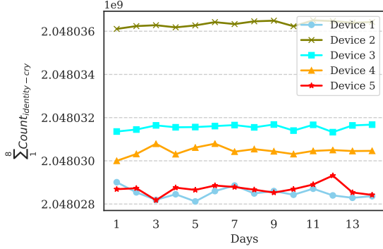
(a) Variation in daily averages of accumulated identity count of crystal oscillator - Count_{identity-cry}
