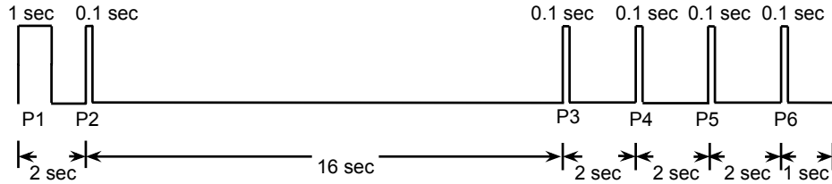
Fig. 9. Timing of audio pulses
