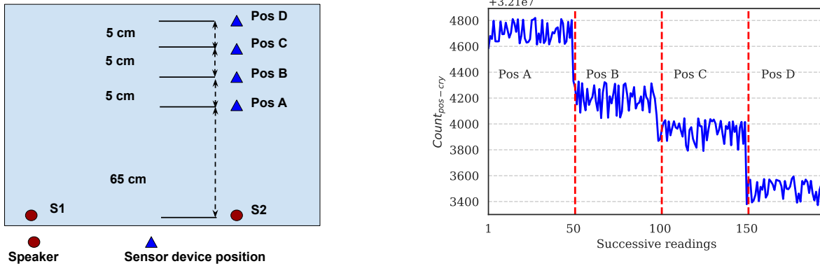
(a) Setup to evaluate the sensitivity of Position_{signature} (b) Position_{signature} at different positions
