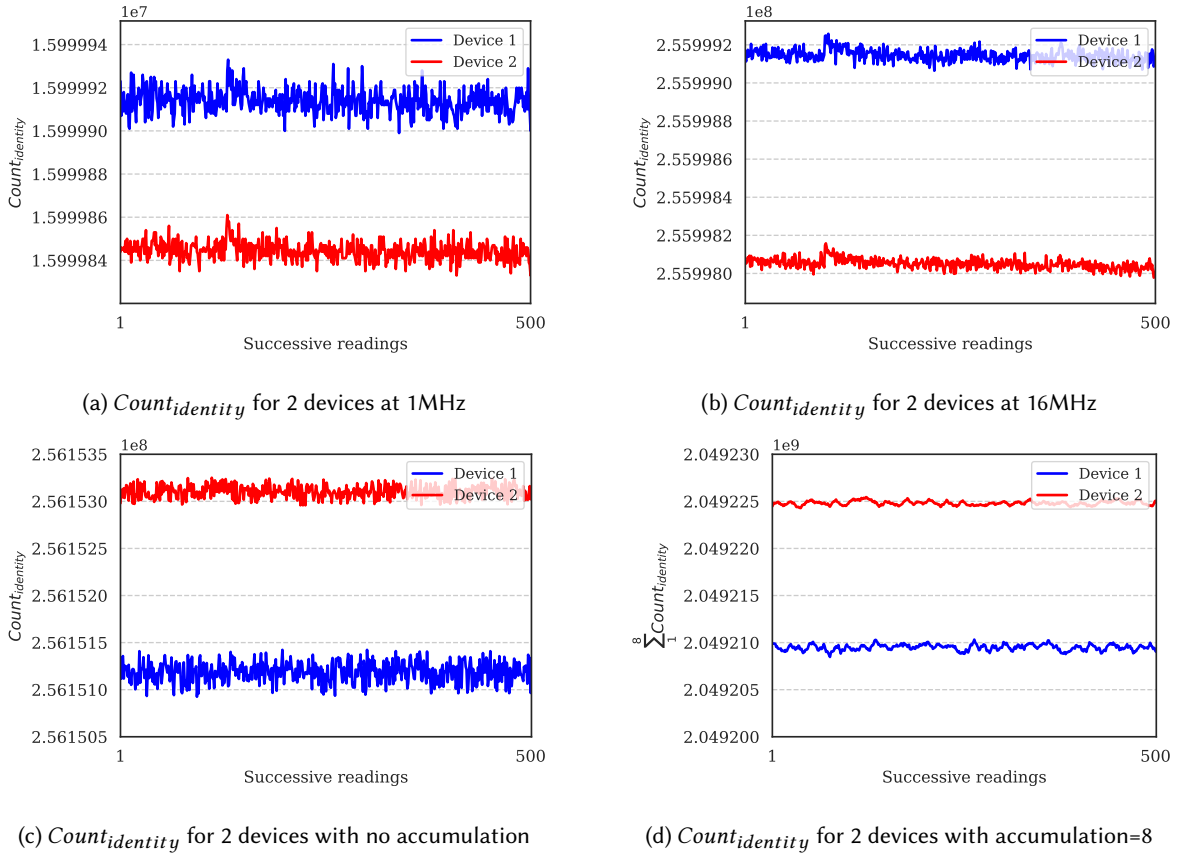
Fig. 4. Impact of timer frequency and accumulation on Count_{identity}
