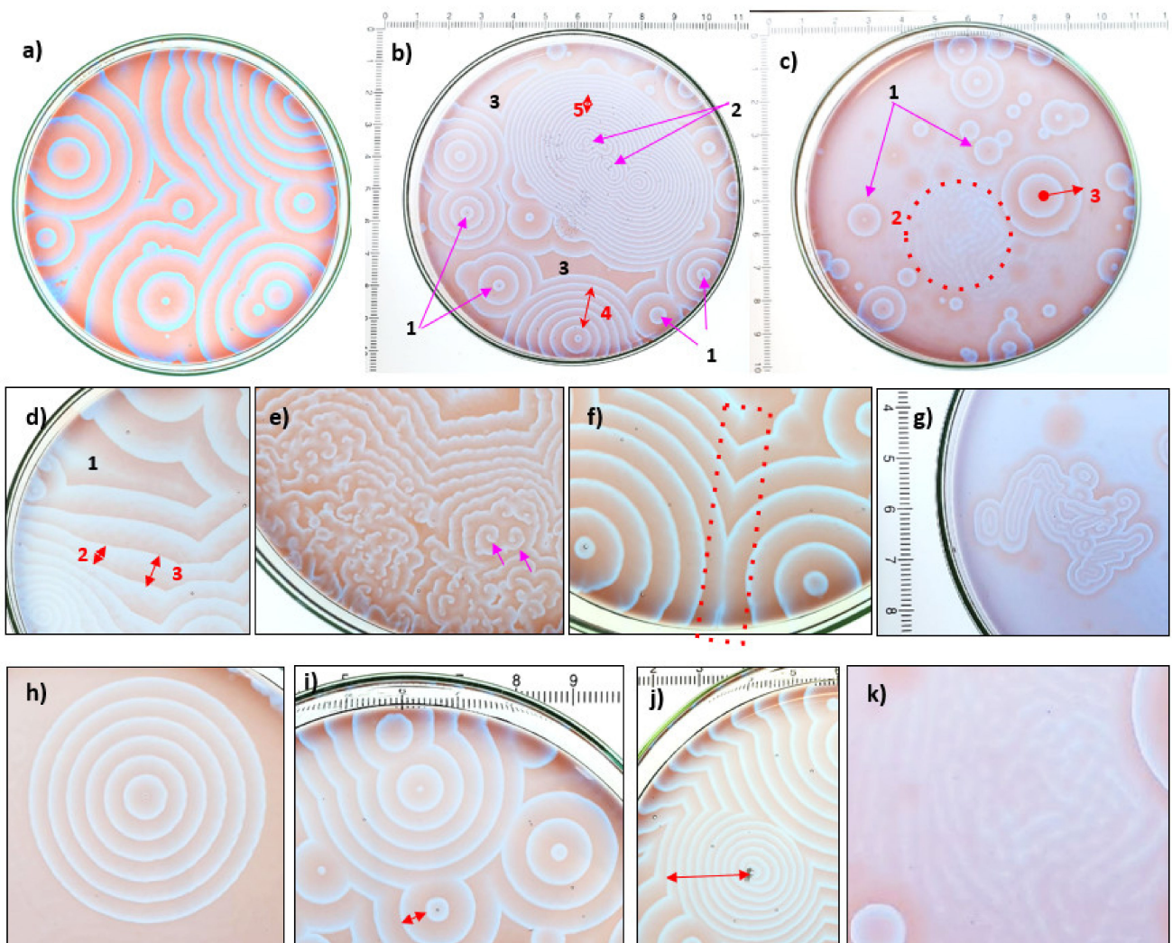
Figure 2. The most common types of self-similar patterns produced for this work by the classical B-Z reaction in Petri dishes 10 cm in diameter.
