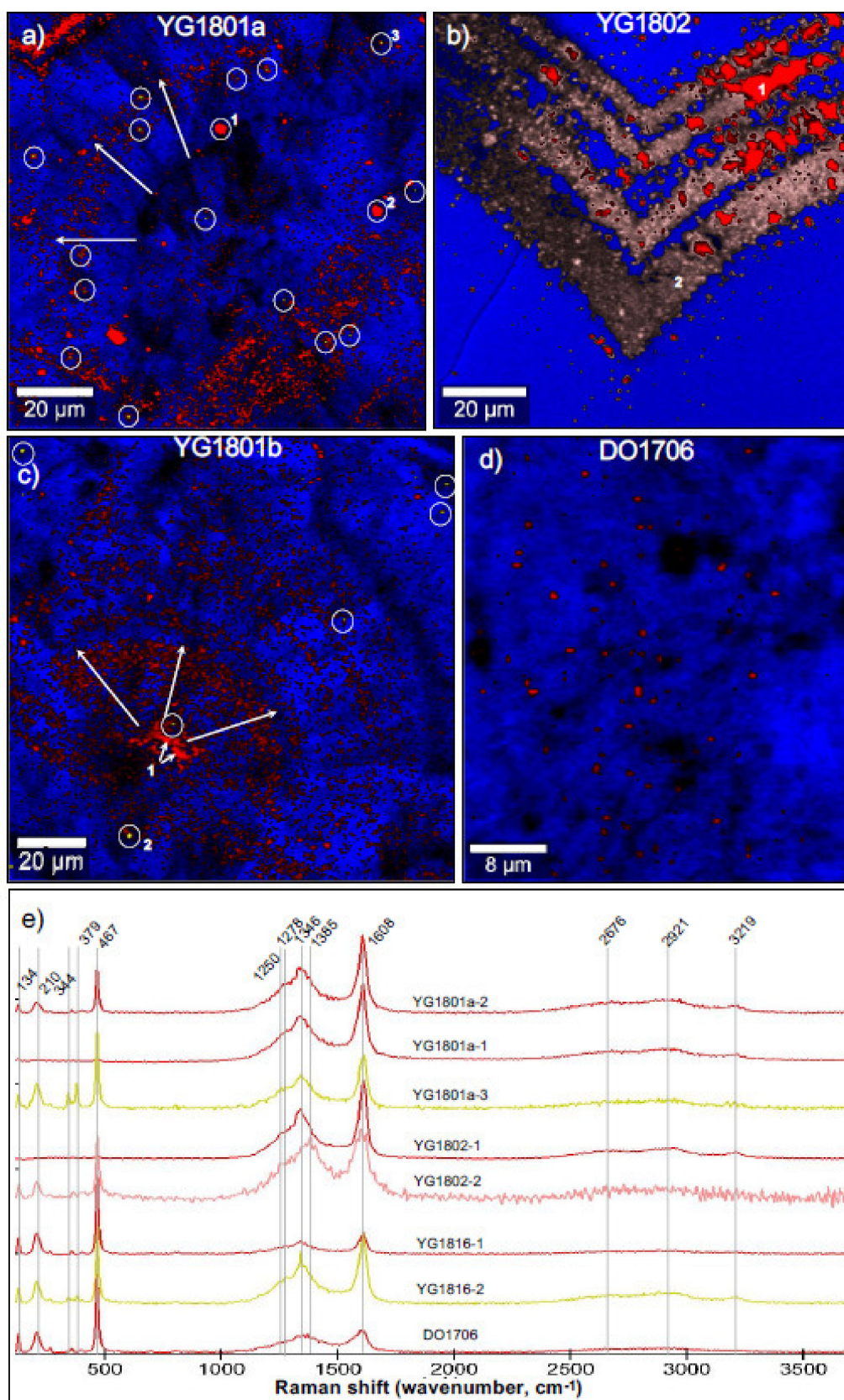
Figure 7. Raman hyperspectral images of organic matter in Doushantuo cap carbonate member 1. (a) Hyperspectral image of organic matter (red) associated with radially aligned acicular quartz (blue) and nanoscopic pyrite (yellow) (YG1801a, Jiulongwan).
