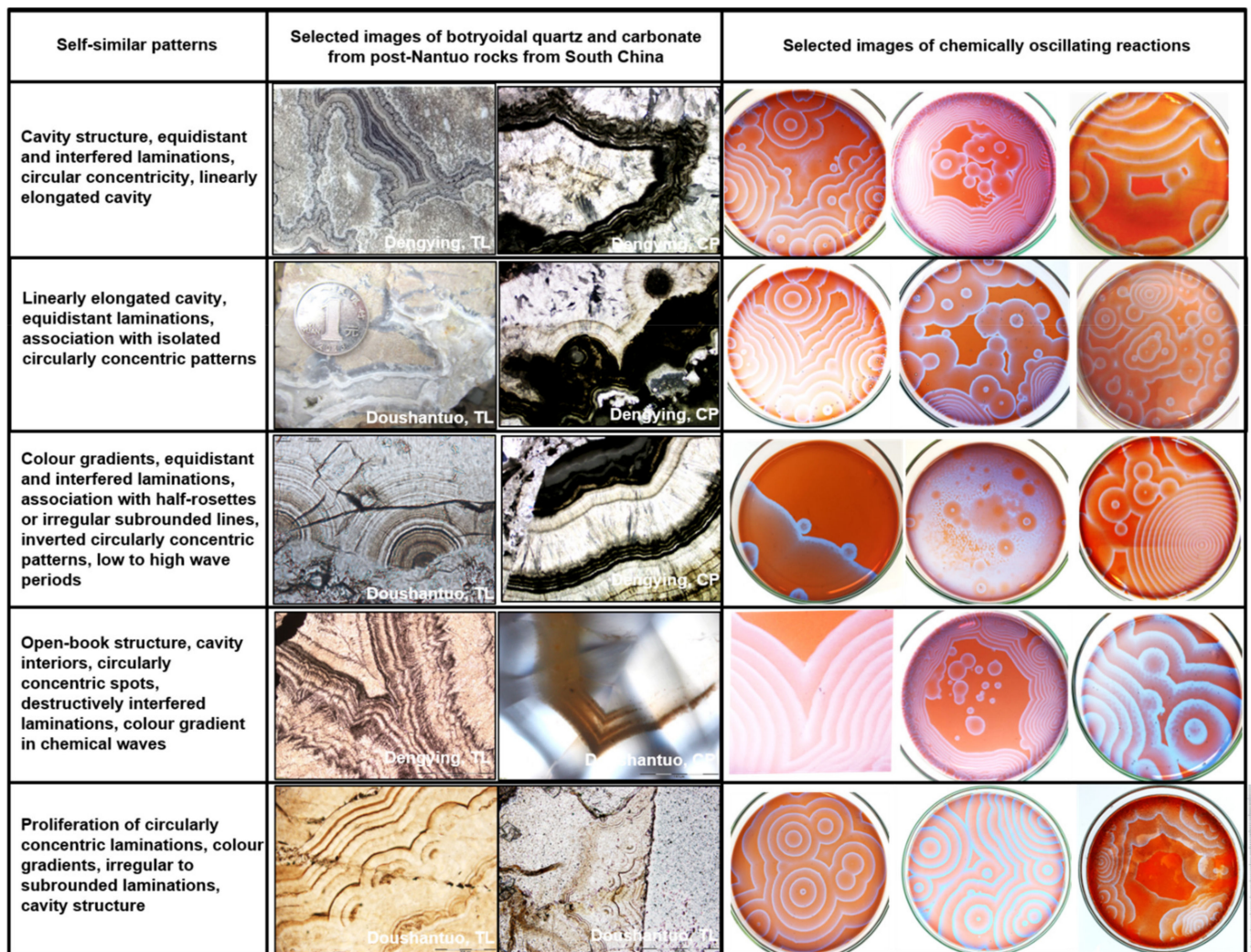
Figure 9. Summative and comparative grid of patterns (Table 1) shared by botryoidal quartz and carbonate, with images from the post-Nantuo of South China, directly compared with selected B-Z experiments, which also produced these patterns. TL is transmitted light (i.e., plane polarized) and CP is cross polarised (i.e., crossed nicols).
