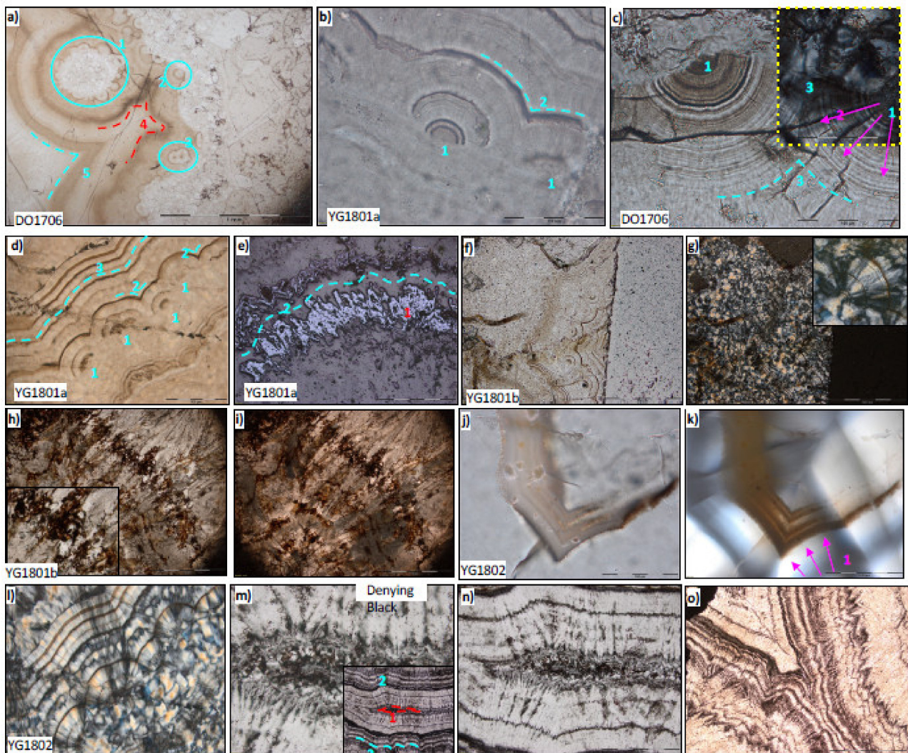
Figure 6. Microscopy images of the studied samples. (a) plane polarised light image of a section of DO1706 showing features of spherical botryoids as clusters onto a large central botryoid (1), lone circular botryoids (2), pairs of botryoids growing close together (3), cavity structure (4), and open book structure with intersected circularly concentric laminations (5). (b) plane polarised image of a section of YG1801a showing features of part botryoids (1) and open book banding intersection (2). (c) Plane polarised light image of a section of DO1706 where the inside yellow dotted square is the cross-polarised light image of the same section of rock superimposed onto the main image. There are features of part botryoids (1) in both plane and cross polarised light with the magenta arrows (2) that indicate the radial crystal growth pattern direction. Note that in cross-polarised light there is a clear line of the intersection (3) between the two botryoidal growths where they form an open-book structure. (d) Plane polarised light image of YG1801a showing botryoids (1) associated with curved laminations formed of intersected circularly concentric laminations. (e) Reflected light image of YG1801a that shows a sub-circular layer of sub-radially aligned blades of Fe-oxides (1) with equidistant laminations, and (f–g) Botryoids of fine grained quartz with circularly concentric laminations of organic matter and radially aligned acicular quartz, best seen under cross polars in (g) and in its inset, where darkened ‘iron cross’ domains flare outward and at about 90° from each other, a tell-tale sign of sphericity. (h,i) Plane and cross polarised light images of sub-radially aligned blades of carbonate stained with filamentous black-opaque organic matter (zoom shown in inset for YG1801b), which forms a chaotic band lining the cavity structure. (j,k) open-book structure in coarse quartz and (l) botryoids in fine quartz from YG1802. (m–o) Plane polarised light images from the Dengying carbonate specimen that show an elongated cavity (1) formed from sub-parallel bands (2) in the fabric of radial, bladed carbonate crystals (note high order interference colours in inset of m), which are coated with black organic matter concentrated specifically along grain boundaries and inside the cavity structure (m–n). As seen in the quartz specimens from the Doushantuo Fm, laminations are contrasted by the variable concentrations of disseminated organic matter, which yield colour gradients in laminations (seen in o).
