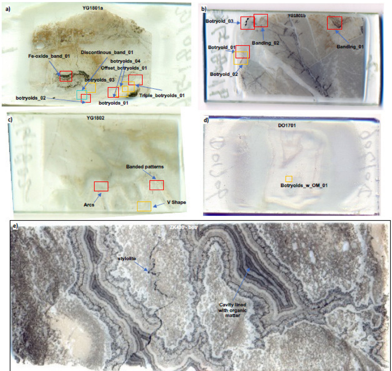
Figure 5. Transmitted light images of the thin sections of the studied rock samples. (a) and (b) Thin sections of two sub-samples of the heterogeneous Doushantuo quartz botryoids (YG1801). (c) Quartz botryoids from another cavity from the Doushantuo member I (YG1802). (d) botryoidal quartz from ‘sheeted cracks’ (DO1701). (e) Botryoidal dolomite from the Dengying Formation (ZK430-botr). All thin sections are 2.5 cm wide (vertical direction). Botryoid targets analysed in this work are shown in red outlines (polarising microscopy) and orange outlines (micro-Raman).
