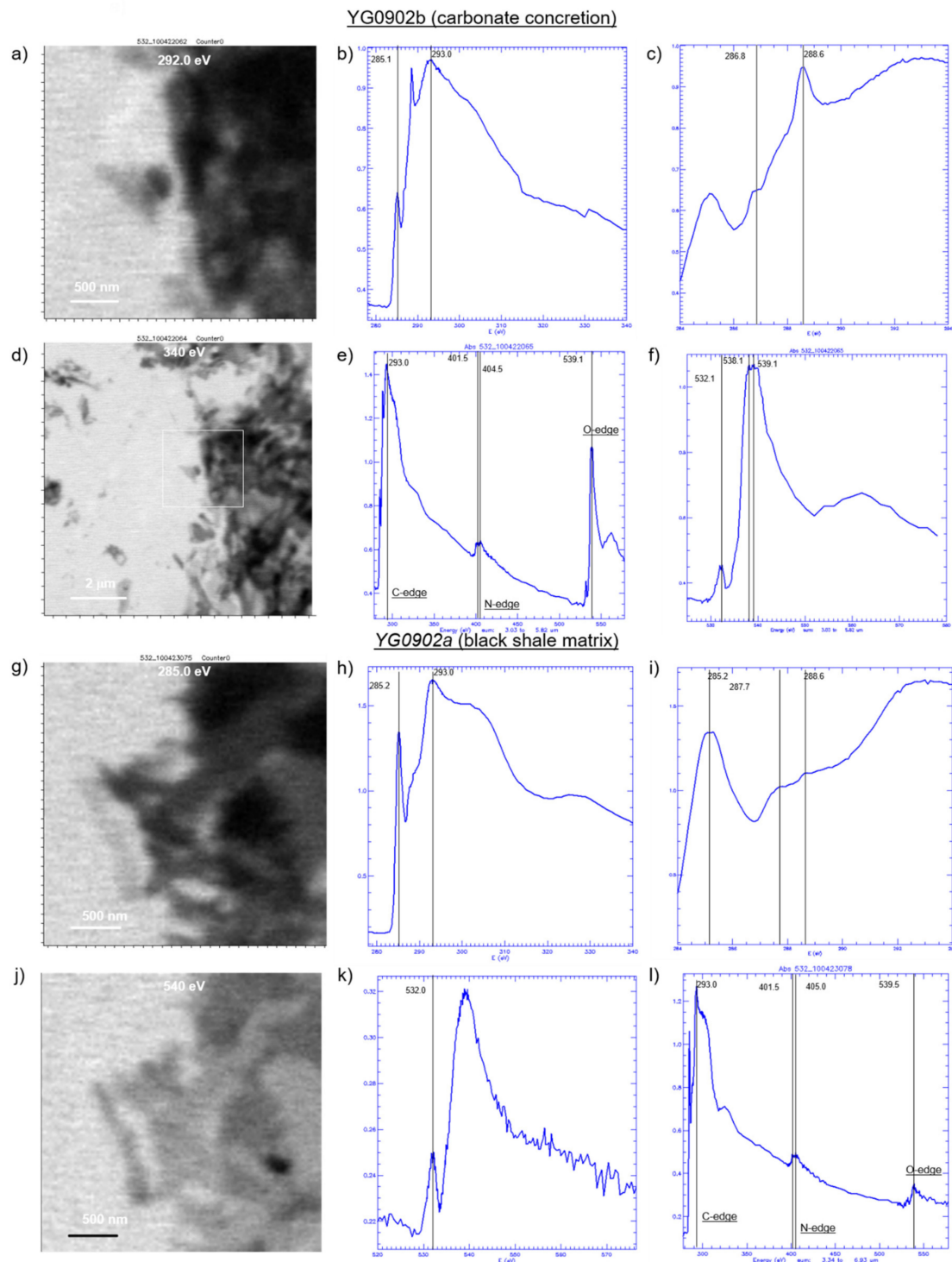
Figure 8. X-ray images and spectra of organic matter extracted from Niutitang black shale. For the carbonate concretion: (a) STXM image at 292.0 eV showing strong absorption of light by the organic matter, (b) C-EXAFS region with the two main edge peaks at 285.3 and 293.0 eV, (c) C-XANES spectrum with two resolvable peaks identified at 286.8 and 288.6 eV from molecular groups, (d) image at 340 eV showing a variety of contrast in the organic matter, (e) full X-ray spectrum covering the range of the C, N, and O edges, and (f) O-XANES spectrum, which shows three resolvable peaks. For the black shale matrix: (g) STXM image of organic matter at 285.0 eV, (h) C-EXAFS region with the same two main peaks as before, (i) C-XANES spectrum that shows a depressed region with two resolvable peaks at 287.7 and 288.6 eV, (j) STXM image at 540 eV showing at least three different contrast levels of gray shades, (k) O-XANES spectrums showing a peak at 532.0 eV, and (l) full X-ray absorption spectrum over the range of energies for the C, N, and O edges.
