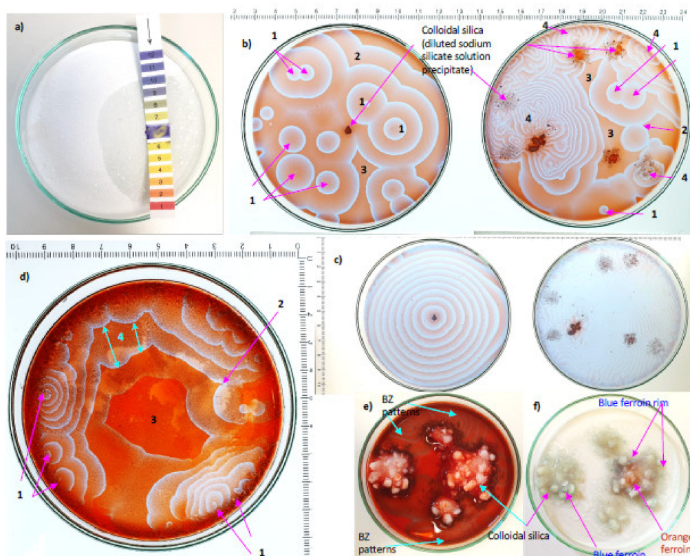
Figure 4. Chemically oscillating reactions in a Petri dish enriched with colloidal silica. Area of uniformly distributed colloidal silica rehydrated with DI water has an alkaline pH of more than 12, as seen on the indicator strip. (b) Classical B-Z reaction with the addition of colloidal silica particles near the centre of the Petri dish. One spatula full of silica scattered throughout the right dish. Both dishes feature point centre oxidation spots (1) and open book features (2) from destructive interference of circular waves along with cavities (3). (a) On the dish to the right with more silica, spirals form (4) with high frequency oscillations, while the waves become irregular. Note the occurrence of spirals in proximity to the silica. (c) Duplicate reactions from “b)” after 40 mins. Note that the colour of ferroin is mostly blue after so long and the strong colour gradients. The left dish is dominated by a single oxidation spot with low frequency oscillations that originate from the central silica particle. The right dish shows the solution is mostly blue with high frequency oscillations self-similar patterns.
