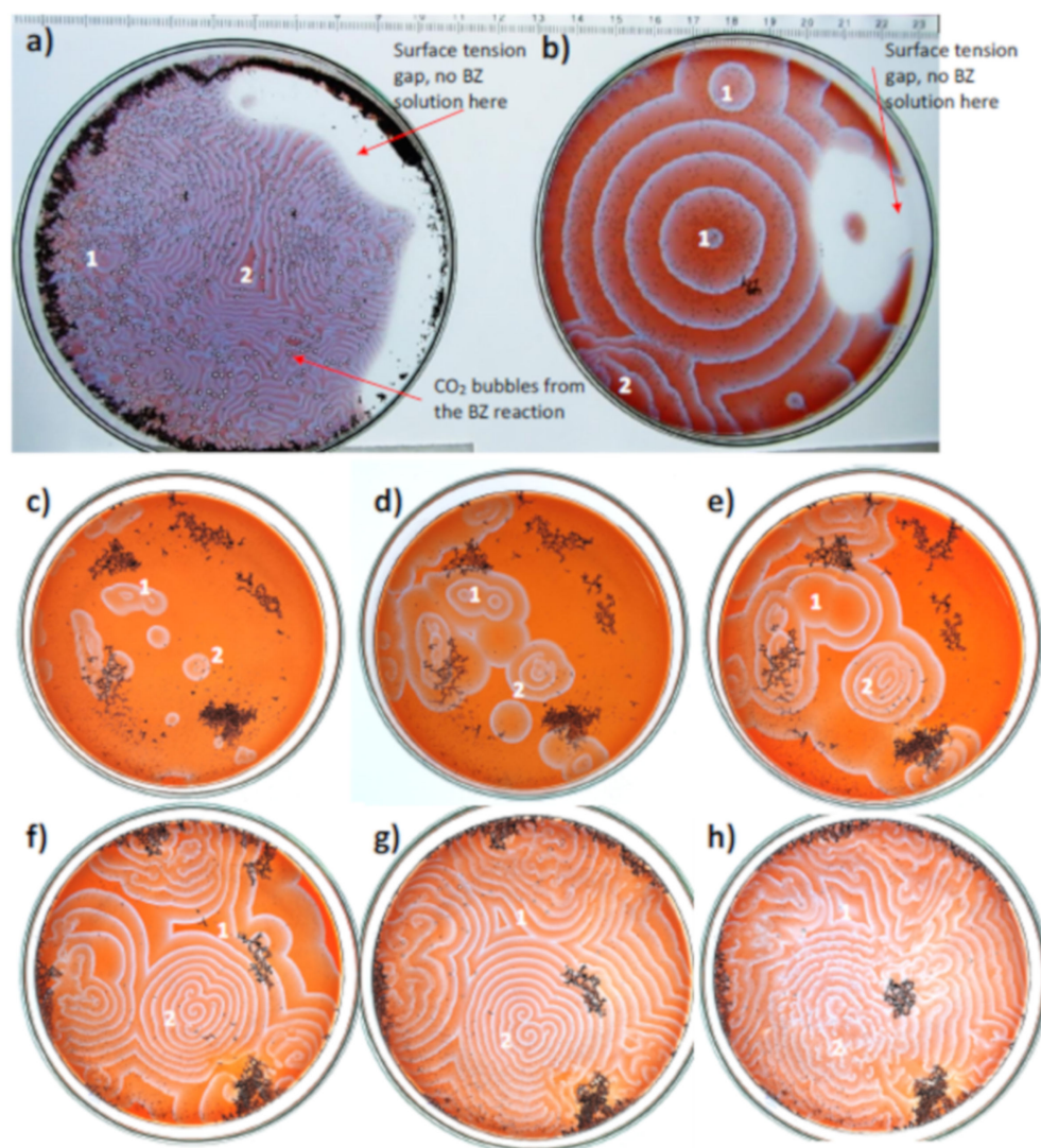
Figure 3. (a) and (b) Standard BZ reaction solution with the addition of humic acid particles (black) in the Petri dish prepared simultaneously. One full spatula of humic acid was initially placed on the dish with the BZ solution poured after. The motion and surface tension of the solution displaced the particles to the edge. This photo was taken after more than 15 min into the reaction and featuring zones of chaotic spiral patterns (1), a large number of \text{CO}_2 bubbles throughout (small white disks with thin black rims), and a closed cavity (2). b) Same experiment with a small amount of particles placed in the centre of the dish with the mixed BZ solution being poured after the addition of humic acid. The experiment was mainly one central oxidation spots with lower frequency waves than Petri dish “a” along with smaller carbon dioxide gas bubbles despite the almost simultaneous start time of the reactions.
