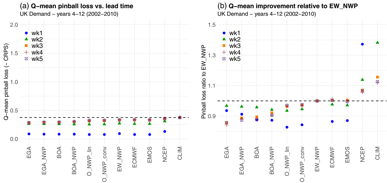
FIGURE 5 (a) UK demand quantile-mean average pinball loss (CRPS estimate) associated with the aggregation rules and the reference forecasts. The average losses for weeks 1–5 are presented as different symbols. The items on the x-axis are sorted from smaller to larger loss based on the week 3 results (orange squares). The dashed horizontal black line shows the value of the week 1 loss for the climatology, as a reference. (b) Relative improvement in skill expressed as relative losses with respect to the EW_NWP combination, for each corresponding week
