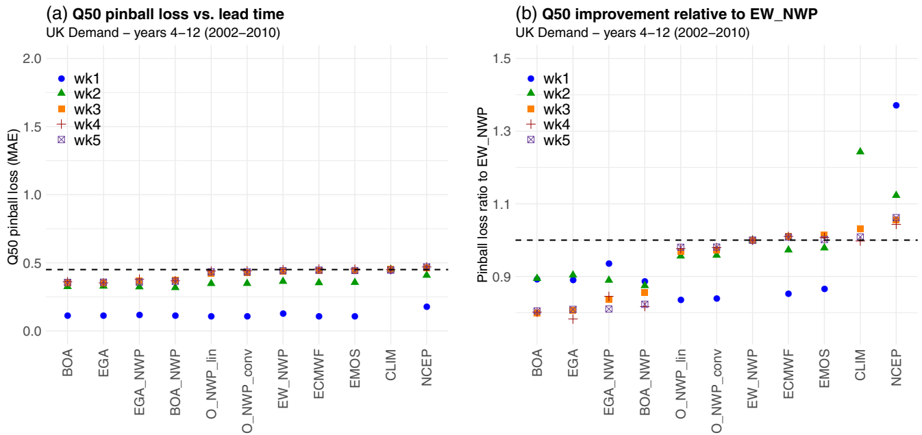
FIGURE 2 (a) UK demand Q50 average pinball loss associated with the aggregation rules and the reference forecasts. The average losses for weeks 1–5 are presented as different symbols. The items on the x-axis are sorted from smaller to larger based on the week 3 results (orange squares). The dashed horizontal black line shows the value of the week 1 loss for climatology, as a reference. (b) Relative improvement in skill expressed as relative losses with respect to the equal-weights combination (EW_NWP) for each corresponding week
