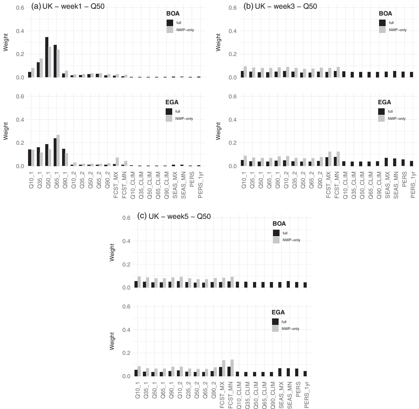
FIGURE 3 Average weights obtained for the UK demand Q50 aggregation rules of the BOA and EGA algorithms over weeks (a) 1, (b) 3, and (c) 5. The black bars correspond to the combinations that consider all the predictors and the gray bars to the NWP-only aggregations. Predictors identified with _1 correspond to the ECMWF system and those marked with _2 to the NCEP system
