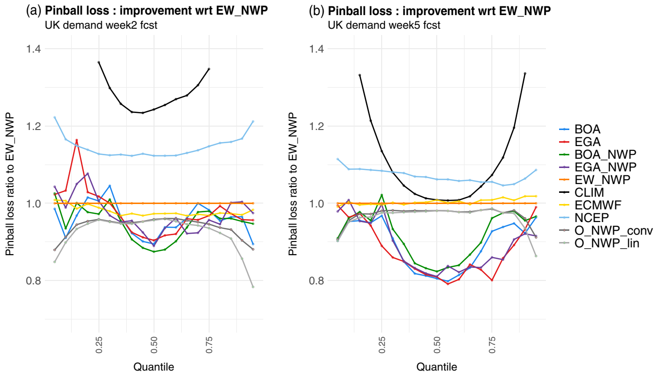
FIGURE 4 Average pinball loss as a function of the quantile for UK demand forecasted as (a) week 2 and (b) week 5. Losses are presented as the relative difference with respect to the EW_NWP loss corresponding to each week. The oracles have been marked in gray and hollow dots to highlight them, as they represent an upper bound to the skill of constant-weighted linear combinations
