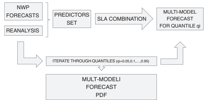
FIGURE 1 Diagram summarizing the application of sequential learning algorithms to combine NWP forecasts and reanalysis into a multimodel probabilistic forecast
