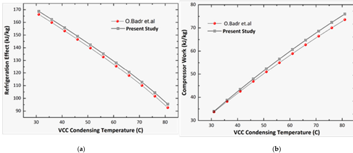
Figure 3. (a) VCC Condensing temperature vs. Refrigeration effect for R22; (b) Condensing temperature vs. Compressor work for R22.
