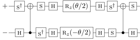
Figure 9: A depth-optimized construction of a single-body term in Fig. 8.
