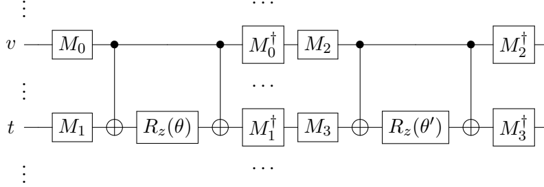
Figure 11: Example circuit for adjacent Pauli string circuits e^{-i\frac{\theta}{2}\sigma_0^v\otimes\sigma_1^t\otimes\cdots}e^{-i\frac{\theta'}{2}\sigma_2^v\otimes\sigma_3^t\otimes\cdots} . Subscripts l to Pauli operators are introduced to conveniently label the associated operators M_l shown in the figure. t denotes the target qubit, v denotes the control qubit, \sigma_l \in \{\sigma_x, \sigma_y, \sigma_z\} , and M_l \in \{\mathbf{H}, \mathbf{s}^\dagger\mathbf{H}, \mathbf{1}\} . If \sigma_l = \sigma_x , M_l = \mathbf{H} . If \sigma_l = \sigma_y , M_l = \mathbf{s}^\dagger\mathbf{H} . If \sigma_l = \sigma_z , M_l = \mathbf{1} .
