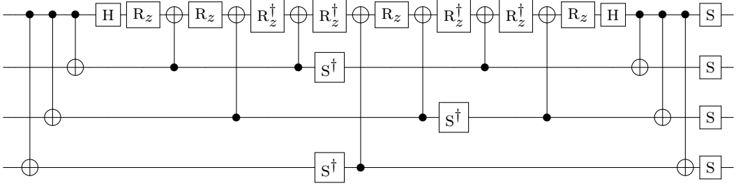
Figure 1: Standard two-body interaction circuit that implements \exp[-i(\theta/2)\sigma_+\otimes\sigma_+\otimes\sigma_-\otimes\sigma_- + \text{h.c.}] . Following the steps detailed in [31] closely, expanding \sigma_+\sigma_+\sigma_-\sigma_- + \text{h.c.} (we suppress \otimes hereafter whenever contextually clear) into the particular ordering of \sigma_x\sigma_x\sigma_x\sigma_x , \sigma_x\sigma_x\sigma_y\sigma_y , \sigma_x\sigma_y\sigma_y\sigma_x , \sigma_x\sigma_y\sigma_x\sigma_y , \sigma_y\sigma_y\sigma_x\sigma_x , \sigma_y\sigma_x\sigma_x\sigma_y , \sigma_y\sigma_x\sigma_y\sigma_x , and \sigma_y\sigma_y\sigma_y\sigma_y , and implementing them one after another with the last qubit as the target qubit, we obtain the circuit shown in this figure after applying the circuit optimization routines detailed in [30, 31].
