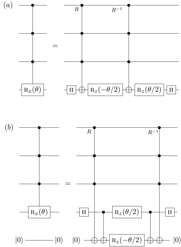
Figure 6: Triply-controlled R_x(\theta) gate implementation with relative-phase triply-controlled NOT gates. The R -prepped triply-controlled Toffoli gate denotes a relative-phase Toffoli gate, i.e., the gate implements a triply-controlled-NOT gate up to relative phases. The R^{-1} -preppendix is used to denote its inverse. The method to implement the relative-phase Toffoli gate is detailed in [7, 27, 28].
