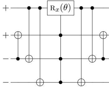
Figure 2: FT-regime optimized circuit for the two-body term e^{-i\theta/2(\sigma_+\sigma_+\sigma_-\sigma_-+\text{h.c.})} . We marked each qubit lines with either + or - to denote which qubits are associated with \sigma_+ or \sigma_- , respectively, for this particular example.
