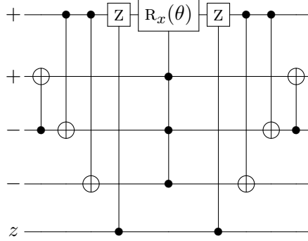
Figure 10: FT-regime optimized circuit for the two-body term e^{-i\theta/2(\sigma_+\sigma_+\sigma_-\sigma_-\sigma_z+\text{h.c.})} . We marked each qubit lines with +, -, or z to denote which qubits are associated with \sigma_+ , \sigma_- , or \sigma_z , respectively, for this particular example.
