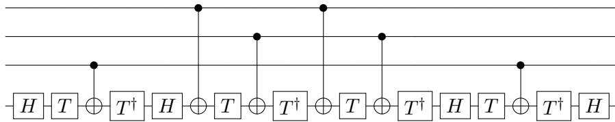
Figure 7: A quantum circuit for a relative-phase triply-controlled NOT gate. The circuit is taken verbatim from [27].
