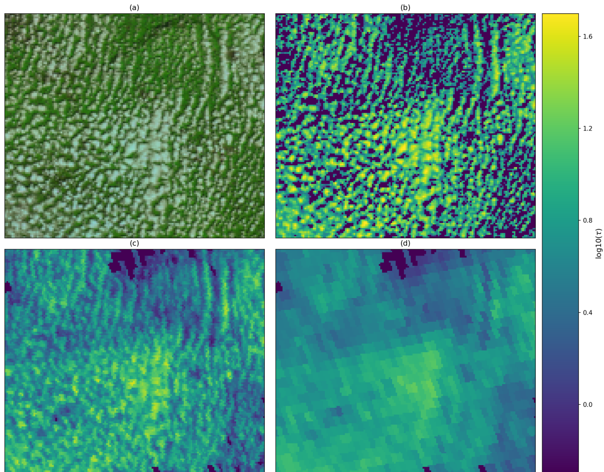
Figure 5. Shallow convective cloud field observed over northeastern France at 3^{\circ}25' \text{E} and 48^{\circ}7' \text{N} on 2 June 2013 at 10:50 Z. MODIS reflectances are displayed as a day-natural color RGB composite in (a), and retrieved values of cloud optical depth ( \tau ) are shown for the operational Terra MODIS C6.1 retrieval (b), the improved Meteosat SEVIRI retrieval (c), and the standard-resolution Meteosat SEVIRI retrieval (d) using a logarithmic color scale.
