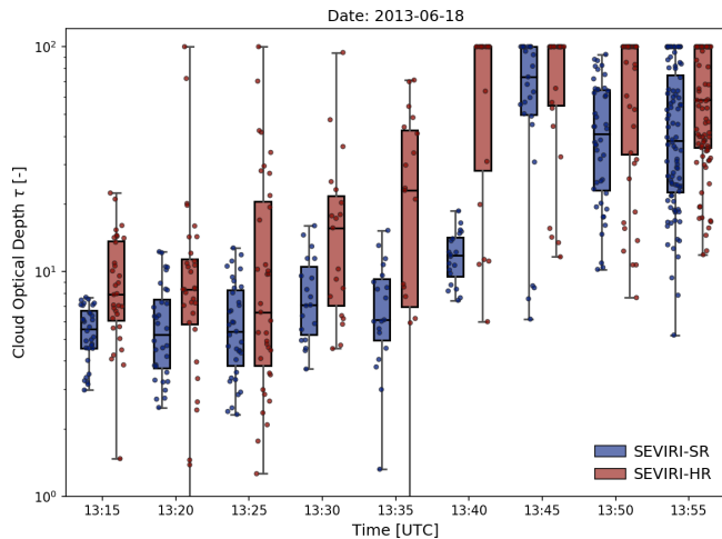
Figure 8. Box-and-whisker plot of cloud optical depth ( \tau ) as a function of time for the convective cell shown in Fig. 7, comparing the standard-resolution retrieval (SEVIRI-SR, blue) and the improved HRV-based retrieval (SEVIRI-HR, red). A time period from 13:15–13:55 Z has been chosen to capture the early growth phase of the convective cell. The boxes extend from the lower to the upper quartile, the lines within the boxes mark the median, and the whiskers extend to the minimum and maximum values of \tau for all pixels belonging to the cloud object. Additionally, points have been added displaying the individual \tau values of the object pixels.
