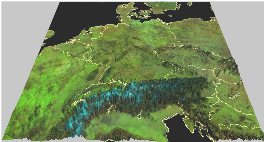
Figure 3. Day-natural color RGB (red–green–blue) false-color composite based on the surface reflectance product of the LSA SAF at wavelengths of 1.6, 0.8, and 0.6 \mu\text{m} used by the improved retrieval scheme. The RGB texture has been overlaid on a three-dimensional perspective rendering of the elevation dataset used by the retrieval, which is derived from the SRTM15_PLUS digital elevation model. Country borders are shown as yellow lines.
