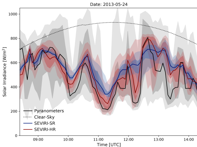
Figure 10. Time series of ground-based and SEVIRI-retrieved surface solar irradiance. The median (thick line), interquartile range (dark shading), and 5th–95th percentile range (light shading) of SSI reported by the 63 pyranometers at the stations in Fig. 9 (black) are shown, visualizing the spatial variability across the stations. The corresponding time series obtained from the standard-resolution (SEVIRI-SR) and the improved HRV-resolution (SEVIRI-HR) SEVIRI retrievals at the station locations are displayed in identical style using blue and red, respectively. All time series have been re-sampled to the 5 min time resolution of the SEVIRI observations. The mean clear-sky irradiance from the satellite retrieval is shown as a dotted black line.
