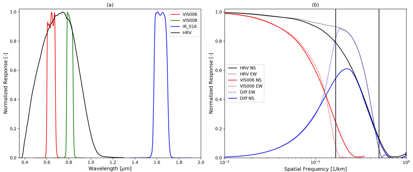
Figure 1. Normalized spectral response of the solar channels of the Meteosat SEVIRI instrument (a). The red, green, blue, and black lines correspond to the 0.6 μm (VIS006), 0.8 μm (VIS008), 1.6 μm (IR_016), and HRV channels, respectively. (b) The modulation transfer function of the HRV (black) and the 0.6 μm (red) channels in the north–south (NS, solid) and east–west (EW, dotted) directions. The vertical black lines show the Nyquist frequency limit of the respective channels depending on their sampling resolution. The differences (Diff) of the two modulation transfer functions in both directions are shown in blue (adapted from Deneke and Roebeling, 2010).
