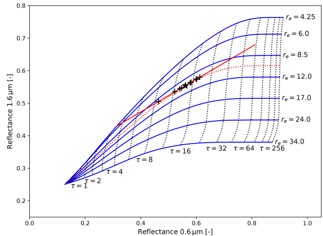
Figure 4. Illustration of the lookup-table-based downscaling method with slope adjustment used in the improved HRV-based retrieval. The relation of the reflectances at wavelengths of 0.6 and 1.6\ \mu\text{m} is shown for contours of pre-calculated cloud optical depth \tau (dotted black lines) and effective radius r_e (solid blue lines) based on detailed radiative transfer calculations. A hypothetical standard-resolution observation with \tau = 14.0 and r_e = 10.0\ \mu\text{m} is marked by the black star. High-resolution retrieval results are marked by black crosses and are constrained to fall on the red line, which is given as tangent to the r_e contour at the point of the standard-resolution observation. See text for further explanation.
