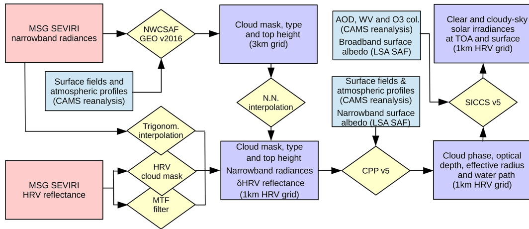
Figure 2. Illustration of the workflow of the improved cloud property retrieval scheme based on observations from the Meteosat SEVIRI instrument at its HRV channel resolution. See Sect. 3 for acronym definitions and further explanation.
