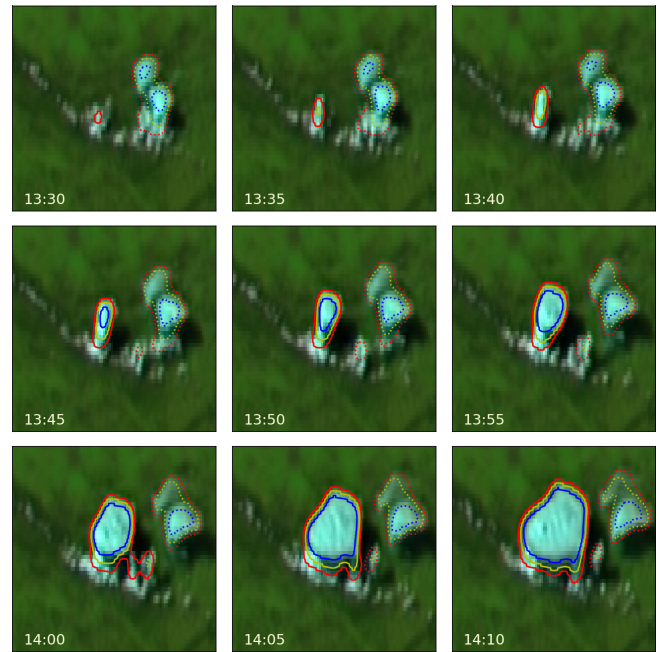
Figure 7. Time sequence of the day-natural color RGB composite showing the SEVIRI reflectances for the 1.6, 0.8, and 0.6 \mu\text{m} channels, downsampled to HRV channel resolution using the constant-reflectance ratio approach described in Werner and Deneke (2020). Frames correspond to a time period from 13:30–14:10 Z on 18 June 2013 and a region of 51 \times 101 pixels (about 100 \times 100 \text{ km}^2 ) centered on the location of convective initiation occurring at 11^{\circ}16'57'' \text{ E} and 50^{\circ}29'30'' \text{ N} . An aspect ratio of 2 : 1 is used to compensate for the lower pixel resolution in the north–south direction. Also shown are contours of the 10.8 \mu\text{m} brightness temperature (red: 273.15 K; yellow: 260 K; blue: 240 K). Solid lines are used for the convective cell of interest, while dotted lines are used for other cells.
