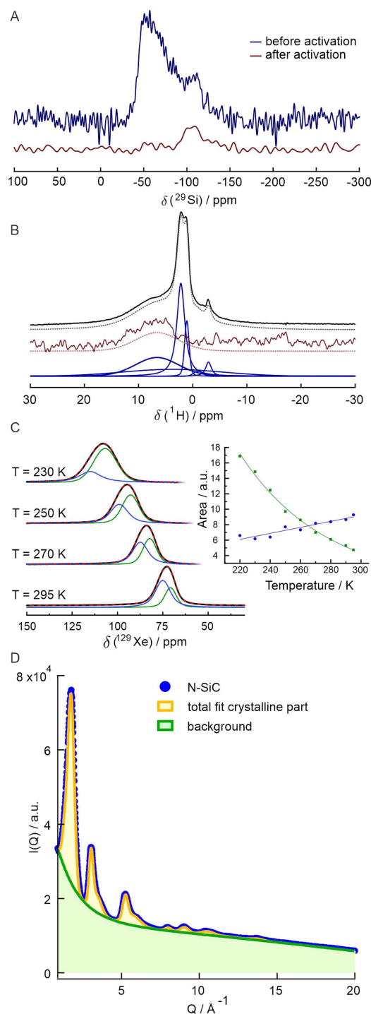
Figure 2. NMR and PXRD/PDF investigations. (A) ^{29}\text{Si} SP MAS NMR spectra of the N-SiC support prior (blue) and after (brown) NaOH treatment (activation). (B) Ultrafast ^1\text{H} MAS NMR spectra; SP excitation (top) and nitrogen selective ^1\text{H}-^{14}\text{N} HMQC excitation (bottom). Both spectra are deconvoluted with the same set of normal components (blue lines). The resulting lineshapes are depicted by pointed lines beneath the experimental spectra (C) Variable-temperature ^{129}\text{Xe} NMR spectra using hyperpolarized ^{129}\text{Xe} within the limiting shift region. The inset depicts the intensity trend for the observed two resonances as function of temperature. (D) PXRD data of N-SiC support material (blue) with its fit for the crystalline phase fraction (yellow) of 17% on the big amorphous background (green).
