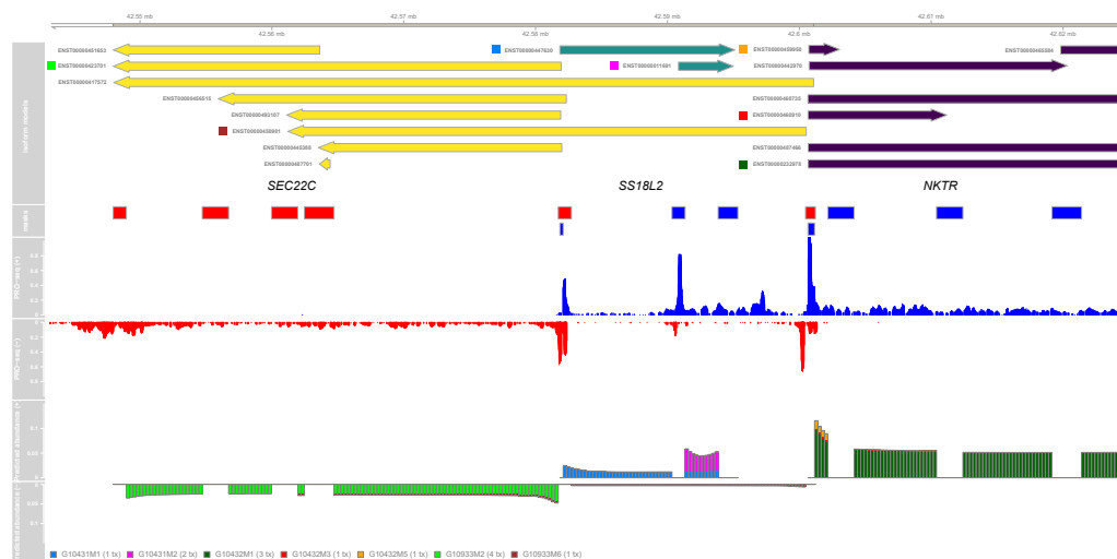
Fig. 3. DENR abundance estimation for three overlapping genes on human chromosome 3. Isoform annotations are shown for SEC22C (yellow; ENSG00000093183), SS18L2 (green; ENSG0000008324), and NKTR (purple; ENSG00000114857), together with the raw PRO-seq signal. The plot at bottom shows the expected relative contribution of each isoform model to the overall read counts per bin. Notice the effect of the shape-profile adjustment near the 5' and 3' ends. Notice also that the PRO-seq data reveals bidirectional transcription near the TSSs of active isoforms; these signals are used by the machine-learning predictor to help identify sequence reads associated with these isoforms.
