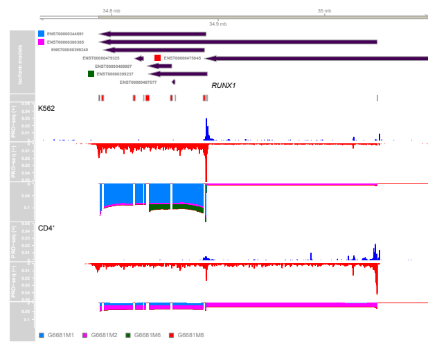
Fig. 4. Cell-type specific TSS usage for RUNX1 . Of several annotated pre-RNA isoforms for the gene encoding the transcription factor RUNX1 on human chromosome 21 (shown on the negative strand at top), DENR finds two isoforms to be dominant: a \sim 100 -kb isoform (G6681M1; shown in blue), and an isoform that is more than twice as long and begins \sim 160 kb upstream (G6681M2; shown in pink). The shorter isoform is clearly dominant in K562 cells (middle), whereas both are expressed at non-negligible levels in CD4 + T cells, with the longer one being slightly dominant (bottom). RUNX1 is essential for normal hematopoietic development and its dysregulation is associated with hematological malignancies Sood et al. (2017). It is well known to make use of alternative promoters Otálora-Otálora et al. (2019); de Bruijn and Dzierzak (2017)
