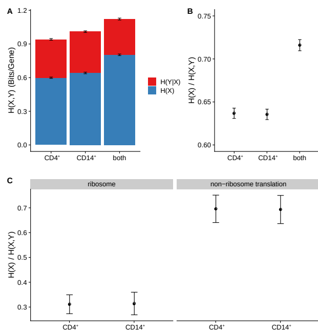
Fig. 5. Decomposition of Shannon entropy of isoform diversity into contributions from primary transcription and post-transcriptional processing. (A) Entropy per gene of mature RNA isoforms ( H(X, Y) ) is partitioned into a component from primary transcription ( H(X) ) and a component from post-transcriptional processing, including splicing ( H(Y|X) ). (B) Fractional contribution from primary transcription, H(X)/H(X, Y) . Results are for 10,650 genes expressed in both CD4 + T cells and CD14 + monocytes. “Both” indicates results when both data sets are pooled. (C) Fractional contribution from primary transcription, as in (B), but for the subsets of genes associated with Gene Ontology terms “ribosome” (left, GO:0005840; n = 135 ) and “translation” (GO:0006412) but not “ribosome” (right; n = 119 ). Error bars represent the standard deviation of the mean as estimated by bootstrap resampling ( n = 100 ).
