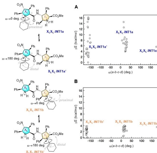
Figure 5. Molecular mechanics Monte Carlo simulations (OPLS 2004 force field) of enamine intermediates X_L X_L - INT1a and X_L X_L - INT1b , in which the relative energies of distal and proximal conformers, defined by the \omega(a-b-c-d) dihedral angles (in absolute value) are shown.
