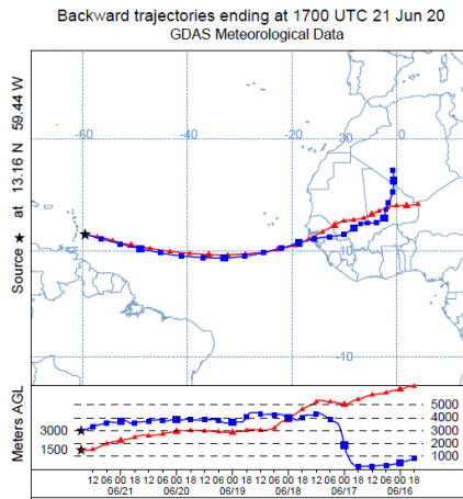
FIG. 4: Backward trajectories with starting point in Ragged Point, Barbados.
