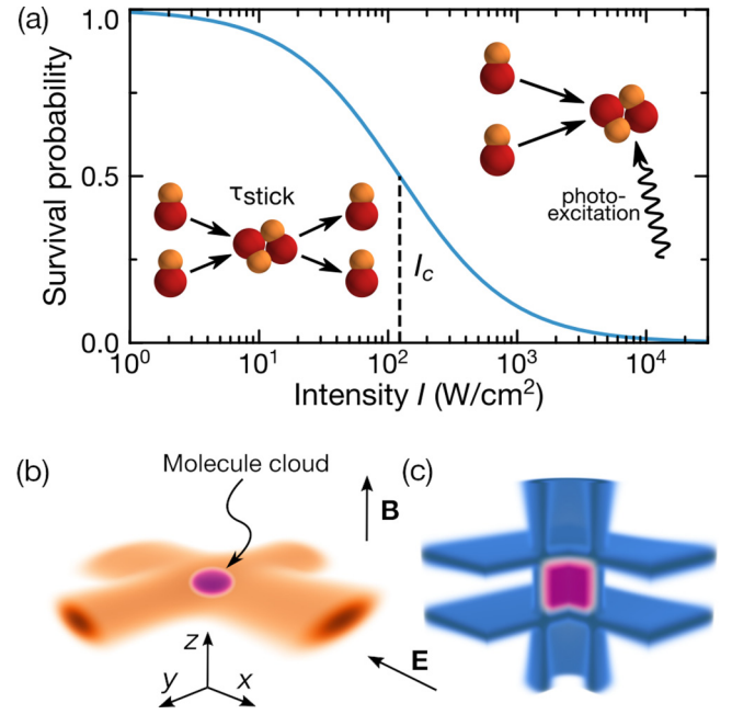
FIG. 1. Overview of sticky collisions and the experimental setup. (a) Probability for two molecules to survive a collision at a given intensity of 1064-nm light according to Ref. [44]. An intermediate sticky complex is formed in every collision, but at high intensity, almost every complex is lost via photoexcitation. Only at low intensity, the complex can decay back into ground-state molecules after a mean sticking time \tau_{\text{stick}} . At the critical intensity I_c , the survival probability is 50%. (b) Red-detuned crossed trap consisting of two elliptical beams of wavelength 1064 nm and 1550 nm. (c) Blue-detuned box trap at 866 nm with vertical cylinder beam and two horizontal elliptical beams. One quadrant is cut out for visibility. The arrows that indicate magnetic field and electric field are valid for both (b) and (c). To compensate gravity in the box trap, we use an electric-field gradient along the z direction.
