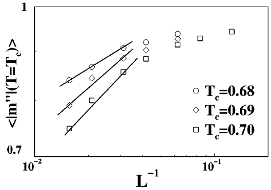
FIG. 11. Log-log plots of \langle m^n(T = T_c) \rangle versus L^{-1} for the mean, maximum, and minimum allowed values of T_c . The linear fits (solid lines) yield an estimate \beta/\nu = 0.16 \pm 0.05 .
