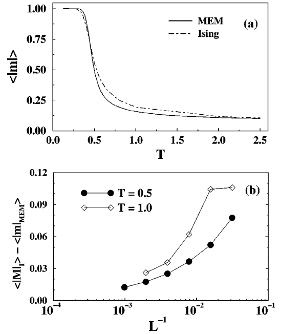
FIG. 3. Comparison of results corresponding to the (1+1)-dimensional MEM and the d=1 Ising model. (a) Plots of \langle |m| \rangle versus T for a lattice of side L = 128 . (b) Linear-log plots of \langle |M| \rangle(L, T) - \langle |m|_{\text{MEM}} \rangle(L, T) versus L^{-1} for T = 0.5 and T = 1.0 . Hence, differences in the magnetization due to finite-size effects appear to vanish in the thermodynamic limit.
