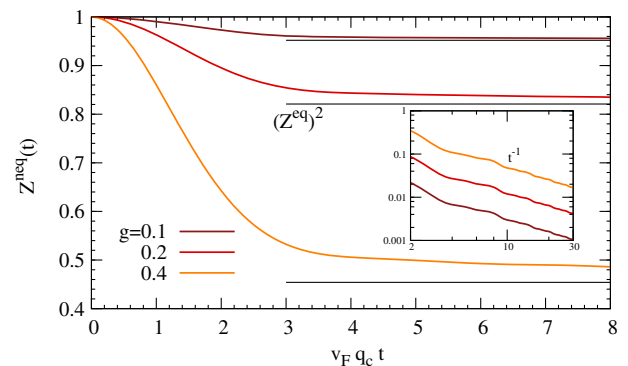
FIG. 1 (color online). Discontinuity of the zero-temperature momentum distribution at the Fermi momentum, Z^{\text{neq}}(t) , as a function of time t for several values of g = f_0 \sqrt{k_F q_c} / (2\pi^2 v_F) . Z^{\text{neq}}(t) exhibits a Gaussian decay at short times. Asymptotically, it saturates to a finite value Z^{\text{st}} \approx (Z^{\text{eq}})^2 (horizontal lines) in the stationary (prethermalized) state. Inset: \ln[Z^{\text{neq}}(t)/Z^{\text{st}}] showing that \ln Z^{\text{neq}}(t) \sim t^{-1} asymptotically.
