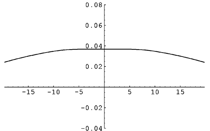
FIG. 1. \langle r^{-4} \rangle_\ell as a function of \nu , for b/a=10 and ka=40 .
