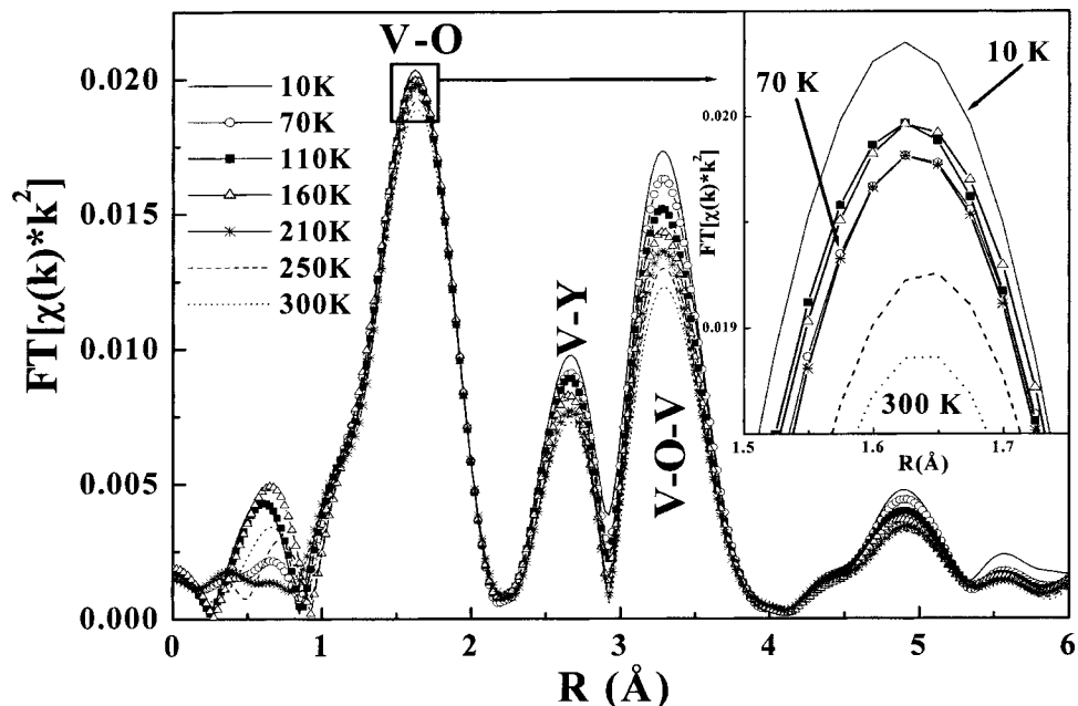
FIG. 3. Fourier transform of EXAFS signal representing the pseudoradial distribution function around V atoms. Inset: Detail of the pseudoradial distribution function for V nearest neighbors.
