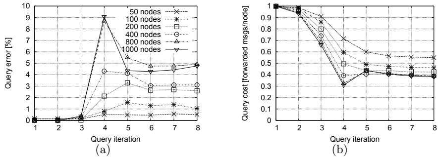
Fig. 4. Adaptation process: (a) Query error and (b) number of transmitted messages in query dissemination in terms of query iteration and network size.
