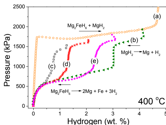
Figure 1. Pressure-composition isotherms (PCI) at 400^\circ\text{C} : (a) complete hydrogenation and (b) dehydrogenation, (c) dehydrogenation of a 1 wt % hydrogenated sample, (d) dehydrogenation of a 2 wt % hydrogenated sample, (e) dehydrogenation of a 3 wt % hydrogenated sample.
