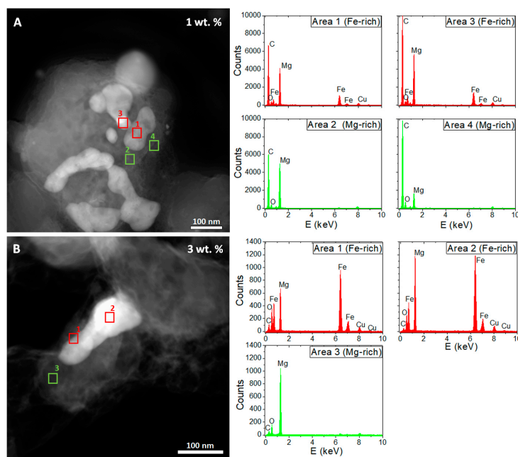
Figure 4. STEM-EDS results for samples after absorption PCI at 400 °C from dehydrogenated as-milled 2\text{MgH}_2\text{:Fe} up to (A) 1 wt % \text{H}_2 , (B) 3 wt % \text{H}_2 .
