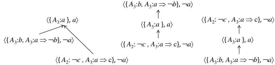
Fig. 2. Three argument trees of Example 6
