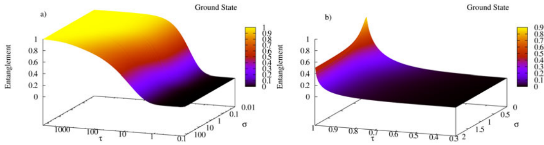
Fig. 3. (Color online) Entanglement of the ground state of the three-dimensional Moshinsky atom with two interacting electrons and a magnetic field. (a) Attractive interaction, (b) repulsive interaction. All depicted quantities are dimensionless.
