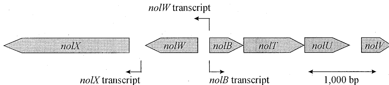
Fig. 1. Map of the cultivar-specificity region nodXWBTUV of Rhizobium fredii strain USDA257.
