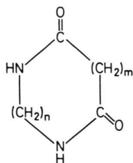
Fig. 1. Dioxodiazacycloalkanes (I) computed. m=2, 3 ; n=2, 3, 4, 5 . Molecular symmetry group is C_{2v} for I ( m=2, n=2 ; m=2, n=4 ) and C_s for I ( m=2, n=3 ; m=2, n=5 ; m=3, n=2 ; m=3, n=3 ; m=3, n=4 ).
