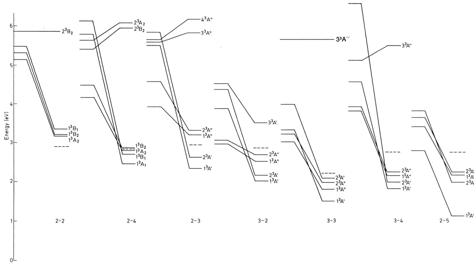
Fig. 2. Singlet-triplet correlation diagram of the lower electronic states of dioxodiazacycloalkanes (I). The symmetry of the spectroscopic states is given by the direct product of the symmetry of the molecular orbitals involved in the transition. See Ref. [4] for the symmetry of the different molecular orbitals. Experimental energies are shown in broken lines.
