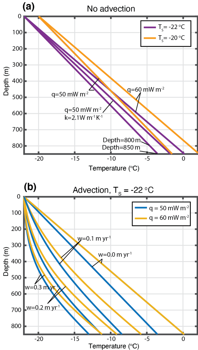
Figure 6. Modeled ice-sheet thermal structure. Panel (a) shows thermal profiles neglecting advection for surface temperatures of T_s = -22\text{ °C} and T_s = -20\text{ °C} . Panel (b) shows thermal profiles including advection for a fixed surface temperature of T_s = -22\text{ °C} . The basal heat flux q is varied between 50\text{--}60\text{ mW m}^{-2} , and the accumulation rate w is varied between 0 and 0.3\text{ m yr}^{-1} .
