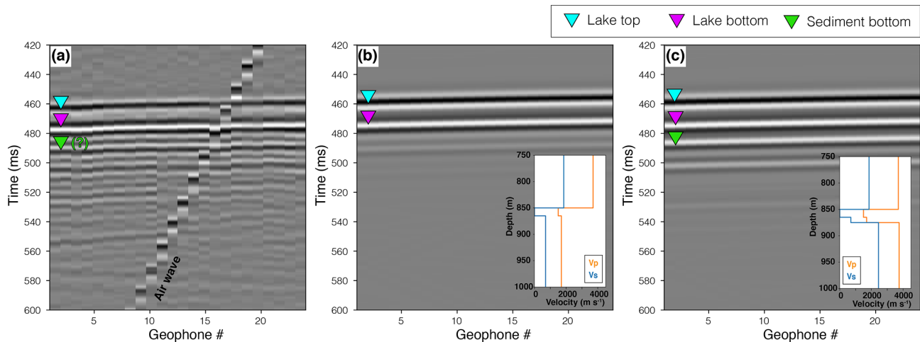
Figure 5. Observed (a) and synthetic (b, c) seismic data for shot gather 12 bandpass filtered between 50–200 Hz. The offset from the source to geophone 1 is 230 m. The colored triangles indicate reflections from the lake top (blue), lake bottom (purple), and sediment bottom (green). The insets in panels (b) and (c) show the V_p and V_s models that were used to compute the synthetics. Both models include a 12 m thick lake below 850 m of ice. The model used in (c) includes an additional discontinuity 10 m below the lake, which represents the boundary between the lake bottom sediments and underlying bedrock.
