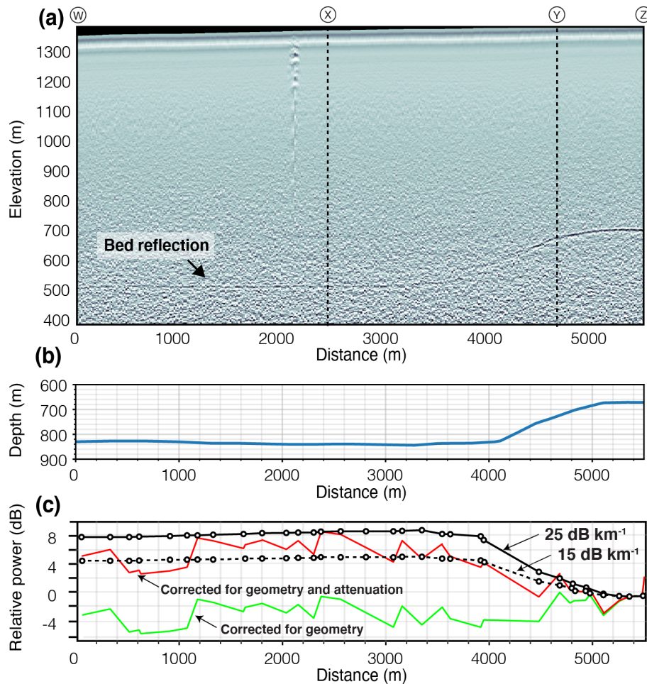
Figure 3. GPR profile. (a) The 5 MHz radar data, unmigrated. The primary bed reflection is marked with an arrow. Vertical dashed lines mark the approximate endpoints of the seismic survey. The depth from the surface to the base of the ice is shown in (b). In panel (c), the relative power of the basal reflections is shown after being corrected for geometric spreading (green line) and both geometric spreading and depth-average attenuation of -15 \text{ dB km}^{-1} (red line). The solid and dashed black lines show the magnitude of attenuation corrections assuming an englacial attenuation of -25 and -15 \text{ dB km}^{-1} , respectively.
