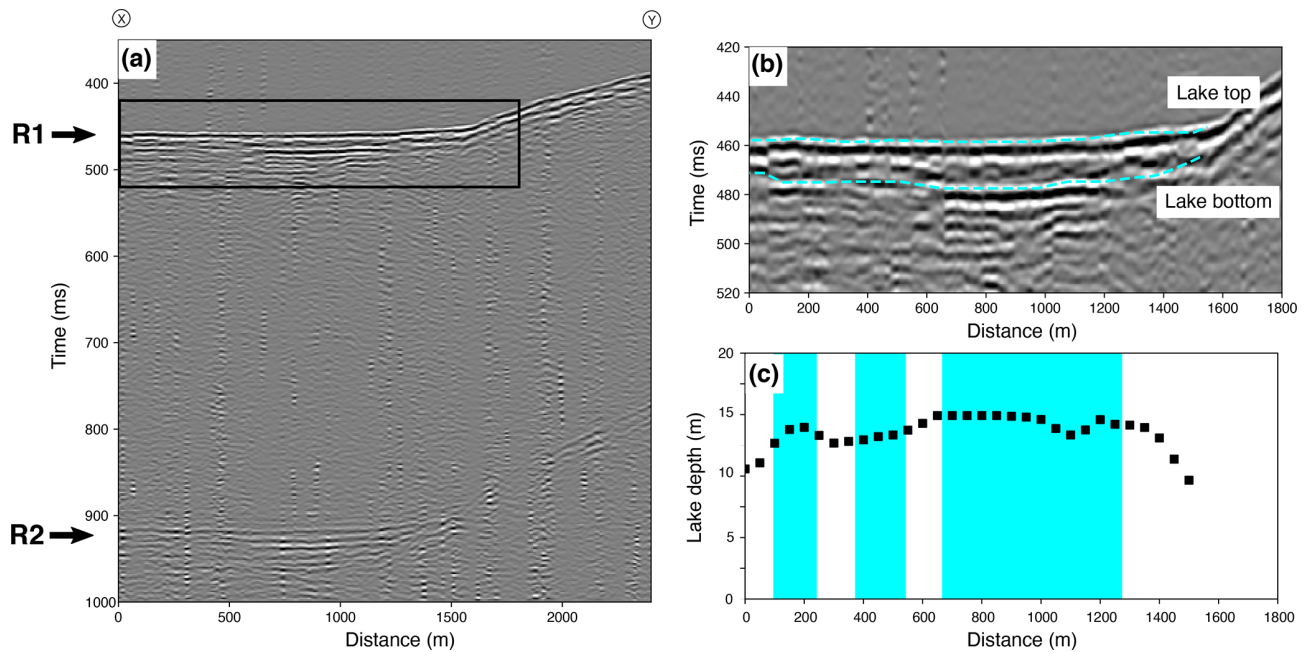
Figure 2. (a) The seismic reflection profile of the entire traverse. Reflections labeled R1 and R2 correspond to the primary reflection from the lake top and its multiple. A transect distance of 0 m corresponds to the southwestern end of the line. (b) A close-up of the R1 reflection window (black rectangle in panel a), showing reflections from both the lake top and the lake bottom. Travel time picks of the lake top and lake bottom reflections are drawn with the dashed blue line. The depth of the lake inferred from the picked reflections assuming a lake V_p of 1498 \text{ m s}^{-1} is shown in (c). Blue-shaded regions indicate where the lake bottom reflection is most clearly identified.
