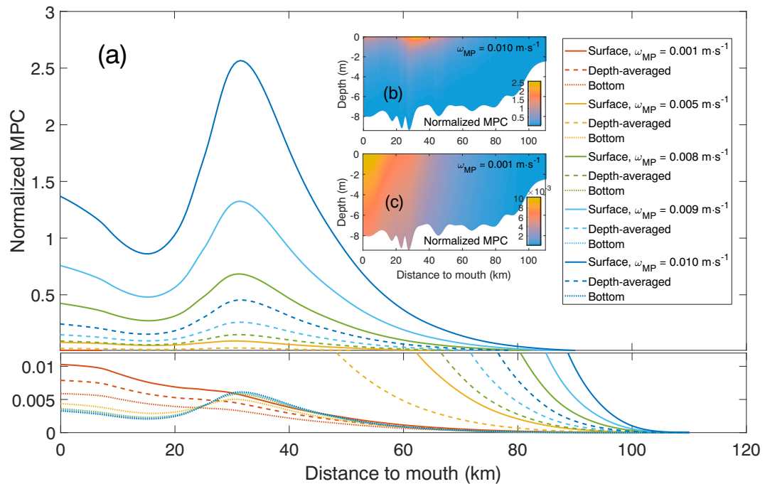
Fig. 7. Surface (solid curves), bottom (dotted), and depth-averaged (dashed) normalized MPC along the main channel of the estuary for different rising velocities, viz. \omega_{MP}=0.001\text{ m s}^{-1} (red curves), 0.005\text{ m s}^{-1} (yellow), 0.008\text{ m s}^{-1} (green), 0.009\text{ m s}^{-1} (light blue), and 0.010\text{ m s}^{-1} (dark blue). Insets (b) and (c) show color plots of normalized MPC for the \omega_{MP}=0.010\text{ m s}^{-1} and \omega_{MP}=0.001\text{ m s}^{-1} cases, respectively. Vertical axis has been split for clarity. (For interpretation of the references to color in this figure legend, the reader is referred to the web version of this article.)
