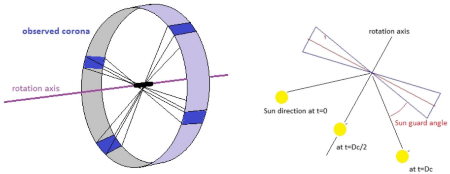
Fig. 1. Left: The 22.5 \times 360 \text{ deg}^2 sky corona swept by the instrument every T_s = 2 \text{ min} (rotation period of the platform 8 min). Right: the same corona is observed during D_c , keeping the Sun away by the guard angle (GA).
