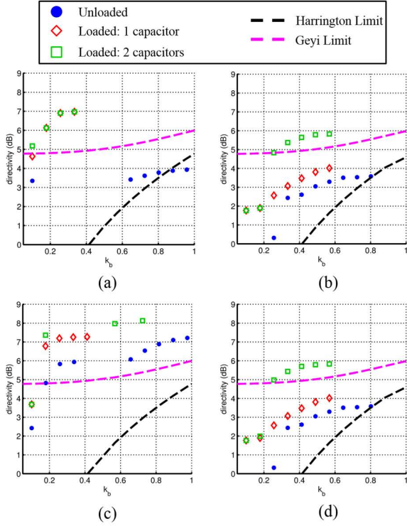
Fig. 7. Pareto fronts of an unloaded gold nanoloop and a gold nanoloop loaded with one or two capacitors. The objectives are minimizing k_b and maximizing directivity along (a) (\theta, \phi) = (90^\circ, 0^\circ) , (b) (\theta, \phi) = (90^\circ, 90^\circ) , (c) (\theta, \phi) = (90^\circ, 180^\circ) and (d) (\theta, \phi) = (90^\circ, 270^\circ) .
