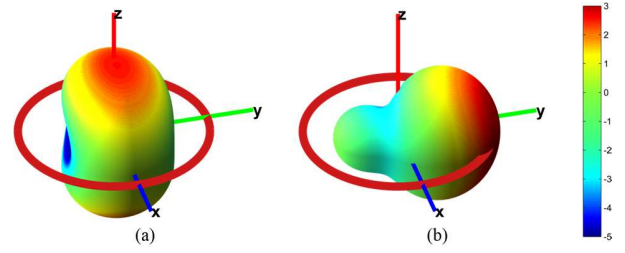
Fig. 12. Comparison of loaded and unloaded gold nanoloop optimized for maximum gain along (\theta, \phi) = (90^\circ, 90^\circ) at k_b = 0.88 . (a) Gain in dB of unloaded loop. (b) Gain in dB of loaded loop.
