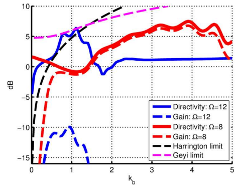
Fig. 6. Comparison of directivity and gain along (\theta, \phi) = (90^\circ, 180^\circ) of a thin ( \Omega = 12 ) and thick ( \Omega = 8 ) circumference loop along with the Harrington and Geyi superdirective limits.
