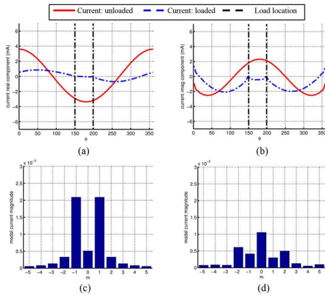
Fig. 9. Comparison of a loaded and unloaded gold nanoloop optimized for maximum directivity along (\theta, \phi) = (90^\circ, 90^\circ) at k_b = 0.88 . (a) Real and (b) imaginary components of the current. (c) and (d) show the modal current magnitudes for the unloaded and loaded cases, respectively.
