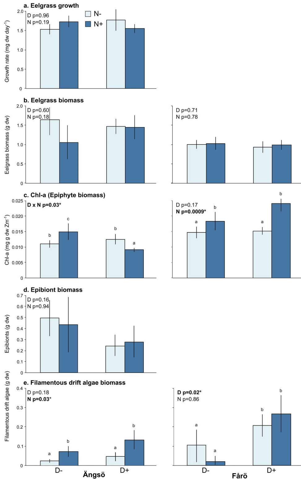
Fig 6. Algal and plant responses (mean \pm SE) in the field experiment: (a) eelgrass growth, (b) eelgrass biomass, (c) chl a (epiphyte abundance), (d) epibiont biomass, and (e) filamentous drift algae biomass at Ängsö (left panel) and Fårö (right panel). Neither eelgrass growth nor epibiont biomass were measured at Fårö 2012. N + = nutrient addition and D + = crustacean mesograzers deterrence. Significant terms are denoted in bold with an asterisk. Significant terms are denoted in bold with an asterisk, and different letters above bars indicate significant differences between treatments ( p < 0.05 ). See Table S3 for full statistical results.
