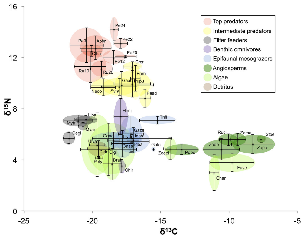
Fig 2. Dual isotope plot ( \delta^{13}\text{C} and \delta^{15}\text{N} ) of the food web in the Ängsö eelgrass meadow. See Table 2 for description of species and material used. Species abbreviations are listed below in alphabetical order by subgroup. Numbers after the perch (Pe) and roach (Ru) abbreviations indicate the size class in cm. Top-predators: Abbr, Abramis brama ; Clha, Clupea harengus membras ; Pe, Perca fluviatilis ; Ru, Rutilus rutilus . Intermediate predators: Ccr, Crangon crangon ; Gaac, Gasterosteus aculeatus ; Neop, Nerophis ophidion ; Paad, Palaemon adspersus ; Pomi, Pomatoschistus minutus ; Pupu, Pungitius pungitius ; Syty, Sygnathus typhle . Filter feeders: Cegl, Cerastoderma glaucum ; Liba, Limecola balthica ; Myar, Mya arenaria ; Mytr, Mytilus trossulus . Benthic omnivores: Chir, Chironomid larvae; Hedi, Hediste diversicolor . Epifaunal mesograzers: Gaoc, Gammarus oceanicus ; Gasa, Gammarus salinus ; Gazo, Gammarus zaddachi ; Idba, Idotea balthica ; Idch, Idotea chelipes ; Hydr, Hydrobiidae ( Ecrobia ventrosa , Peringia ulvae ); Thfl, Theodoxus fluviatilis . Angiosperms: Pope, Potamogeton perfoliatus ; Ruci, Ruppia cirrhosa ; Stpe, Stuckenia pectinata ; Zapa, Zannichellia palustris ; Zode, decaying Zostera marina ; Zoma, fresh Zostera marina . Algae: Char, Chara spp.; Clgl, Cladophora glomerata ; Dral, Drift algae; Fuce, Fucus vesiculosus ; Poly, Polysiphonia spp.; Ulva, Ulva spp.; Zoepi, Zostera marina epiphytes. Detr, Detritus. Note that neither phytoplankton nor particulate organic matter (POM), i.e., major food sources for filter feeders, were sampled in this study, but typically have \delta^{13}\text{C} values of -18 to -20 and -25 to -30 , respectively (Gagnon et al. 2013).
