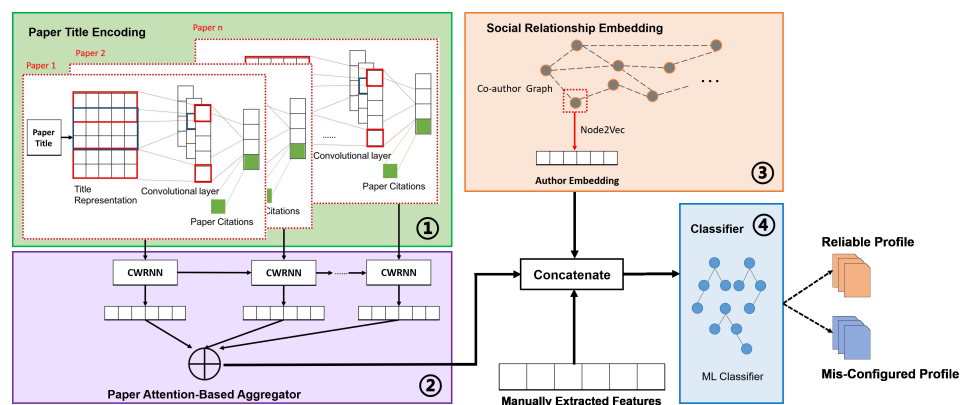
Figure 2. The architecture of the model. (1) The green box (box ①) is the process of paper title encoding where TextCNN is leveraged. (2) The paper attention-based aggregator is shown in the purple box (box ②), where the hidden features of different papers are produced by CW-RNN and aggregated with different weights. (3) The orange box (box ③) shows the process to obtain the author embedding from the co-author graph. (4) The blue box (box ④) is a machine learning classifier (we use LightGBM in this paper) to classify the author profiles based on the concatenated features. (5) The output of the models is the judgment of whether an author profile is mis-configured or not.
