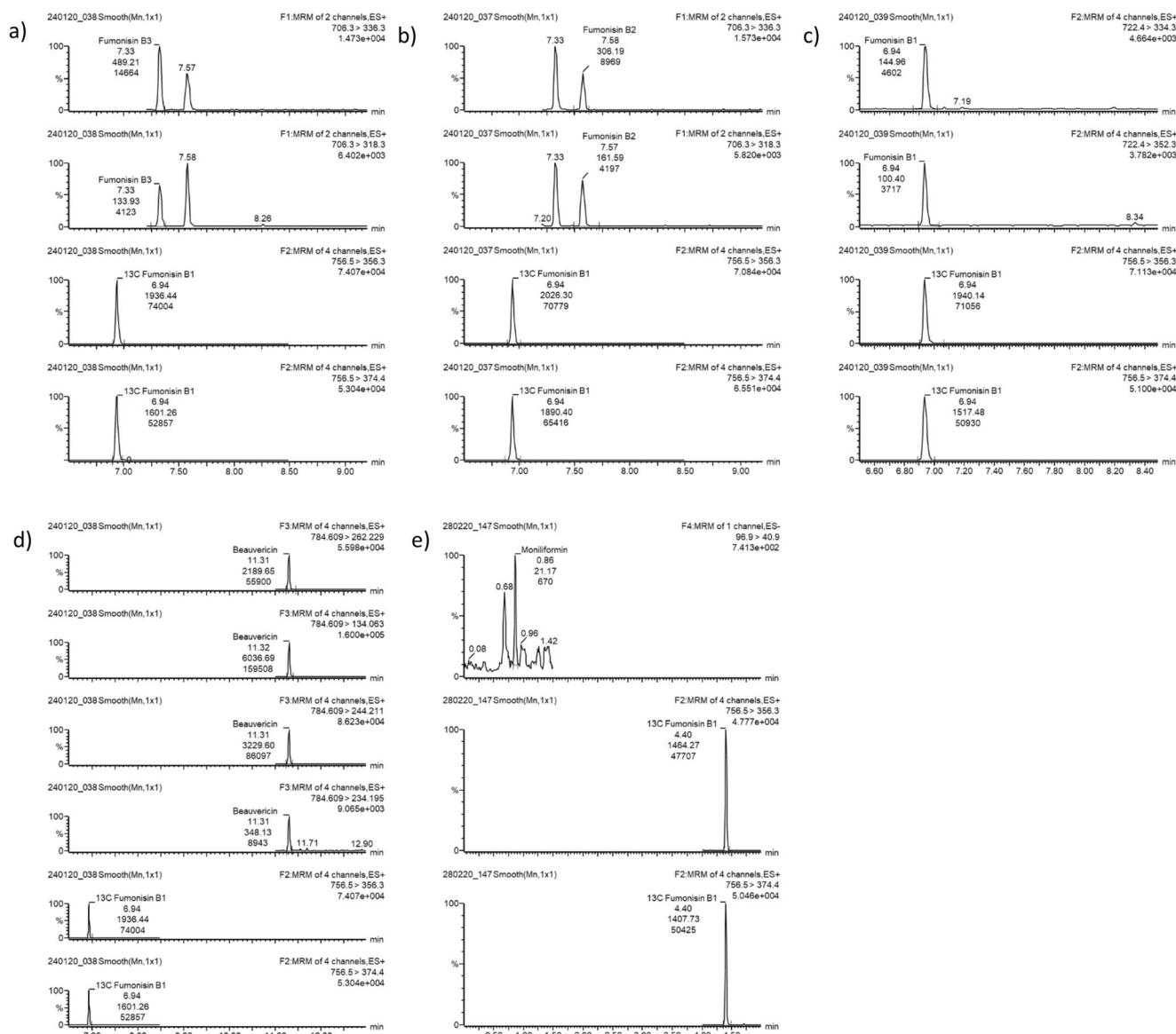
Fig. 1 Multiple reaction monitoring (MRM) chromatograms of the recovery tests with each of the following mycotoxins added at 5.0 ng g -1 concentration in uninfected onion matrix: a fumonisin B 3 , b fumonisin
