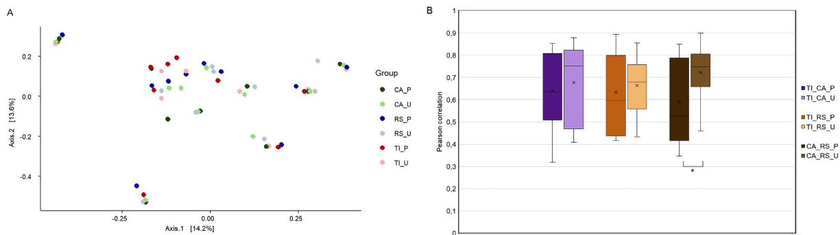
Fig. 3. 16S rRNA gene sequencing data. A – PCoA plot of Bray-Curtis dissimilarities of the 16S rRNA data. B – Comparisons of inter-site 16S rRNA data Pearson correlations between P and U samples of TI, CA and RS. TI_CA_P is an inter-site comparison of the P biopsies of TI and CA, TI_CA_U of the U biopsies of TI and CA, etc. Statistical significance was accepted at p < 0.05 .
