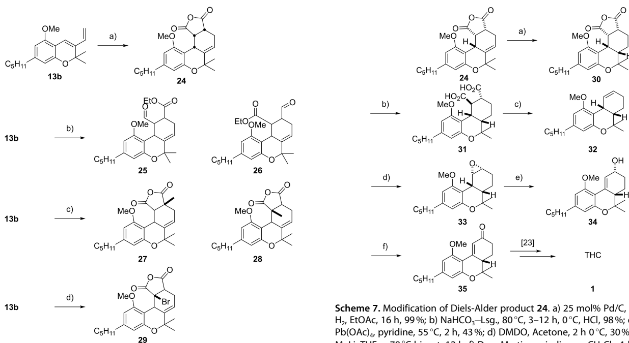
Scheme 6. Diels-Alder reactions with diene 13b: a) maleic anhydride, ACN, 0 °C to r.t., 16 h, 24, quant; b) ethyl (E)-4-oxobut-2-enoate, DCM, 0 °C to r.t., 36 h, 25 14%, 26 7%. c) methyl maleic anhydride, ACN, 0 °C to r.t., 60 h, 27 33%, 28 10%; d) bromo maleic anhydride, ACN, 0 °C to r.t., 36 h, 29 17%, second regioisomer was not isolated.
