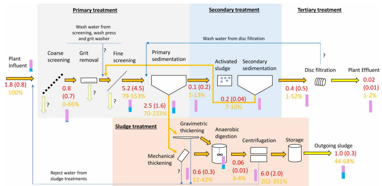
Figure 2 | Microplastic particle loads on the Nenäinniemi WWTP with all the sampled process phases at the plant. Red numbers indicate \times 10^9 microplastics d^{-1} (standard deviation based on three replicates), and orange numbers indicate the average flow normalized to the average MP d^{-1} entering the WWTP. For size-fractionated samples, the highest observed standard deviations are shown. Bars indicate the average proportion (%) of fibers (blue) and fragments (pink).
