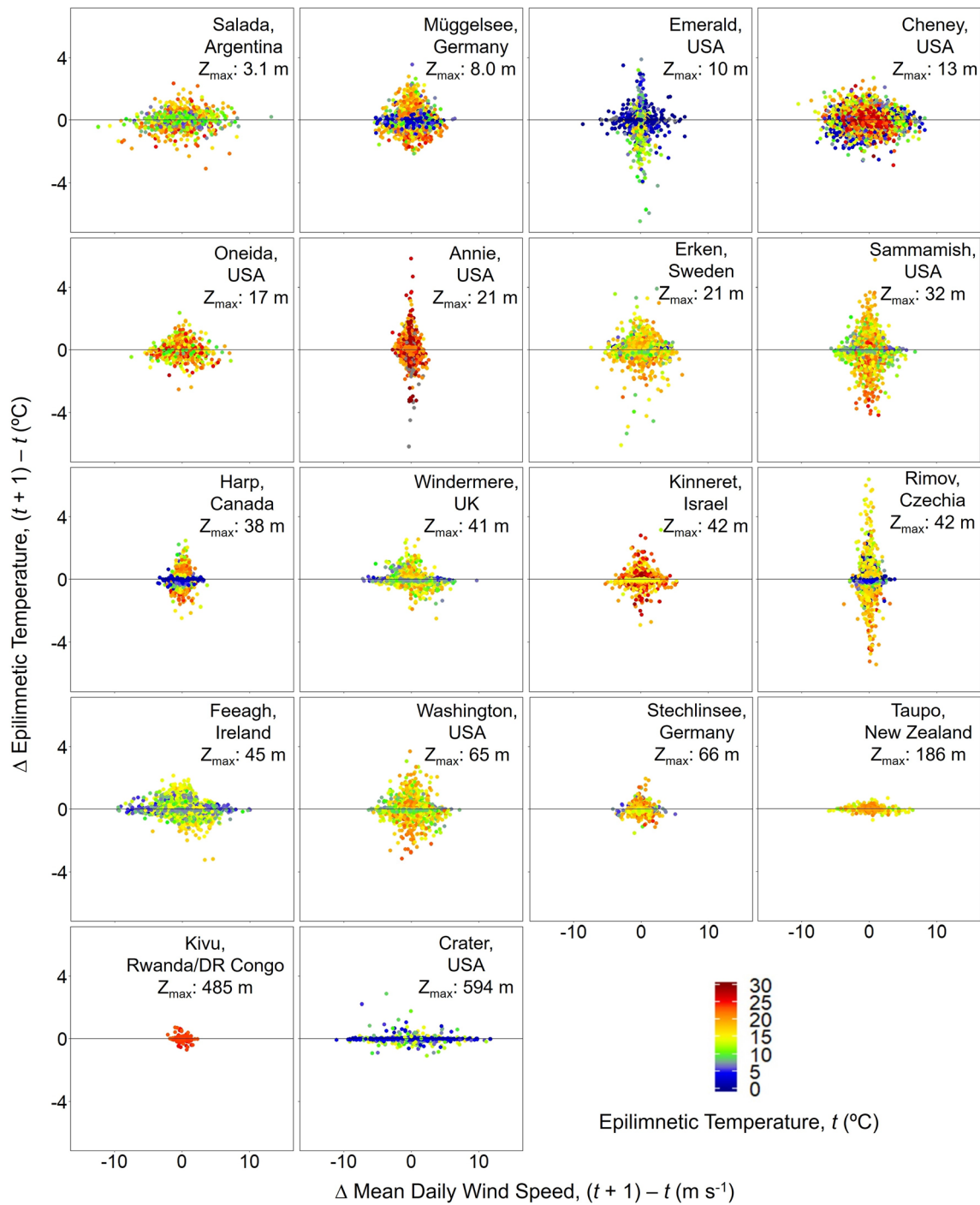
Fig 1. Day-to-day ( [t + 1] - t ) changes in epilimnetic temperature as a function of day-to-day changes in mean daily wind speed ( [t + 1] - t ) across all lakes and all sampling dates. Z_{\text{max}} is the maximum depth (m) for each lake. Colors refer to the epilimnetic temperature at time t when the data were collected.
