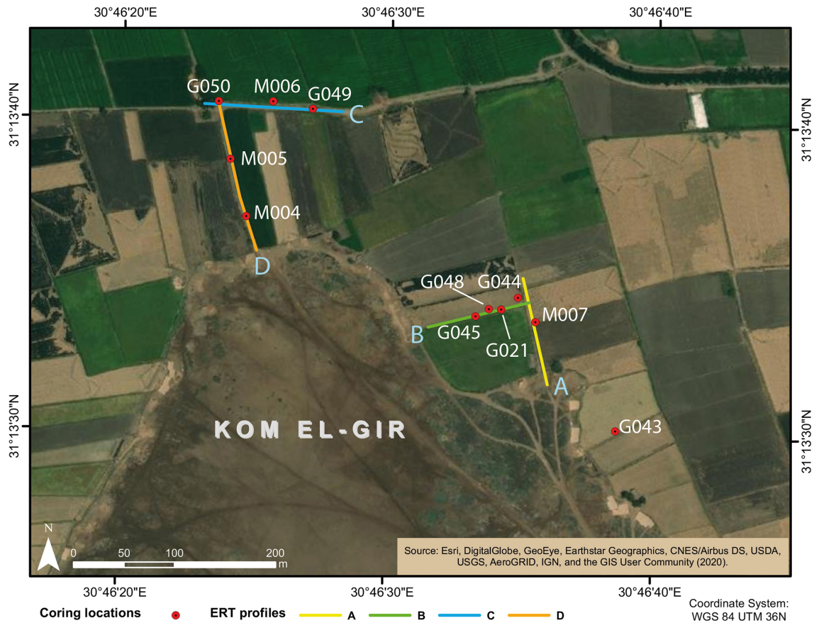
Figure 3. Locations of performed corings and ERT profiles within the study area located north and northeast of KeG.
