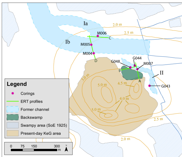
Figure 8. Reconstructed channel systems in the northern and north-eastern surroundings of KeG. Based on topographic map of the Survey of Egypt from 1925 (scale 1 : 25 000).
