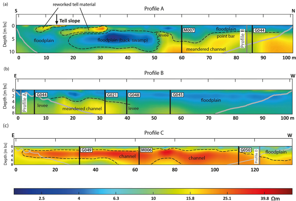
Figure 5. Modeled ERT images of (a) profile A, (b) profile B, and (c) profile C with identified subsurface channel elements. The color scale visualizes the resistivity of the subsurface sediments, ranging from blue, representing low resistivity to red, representing high resistivity. Further features such as locations of several corings conducted in this area are also indicated. The grey lines mark the boundaries of uncertain result reliability towards the start and end of the profile. For profile location see Fig. 3.
