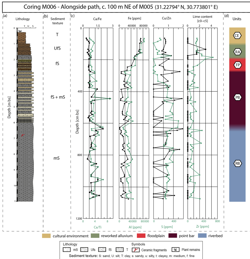
Figure 4. Lithostratigraphy (a) and sediment texture (b) as well as pXRF results of selected proxies (c) for coring M006. For unit interpretation (d) see Sect. 5.
