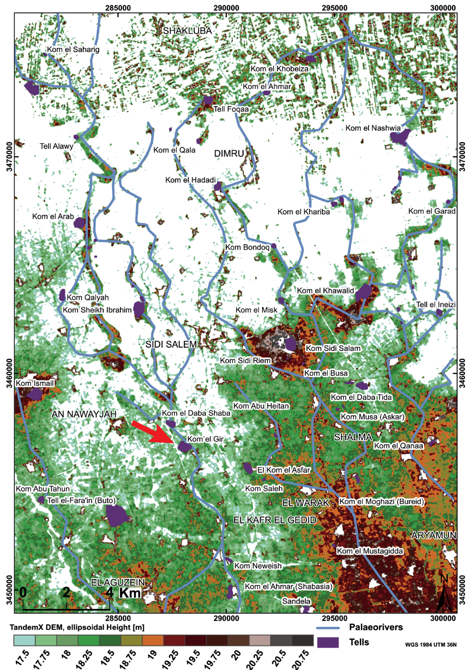
Figure 2. TanDEM-X image of the regional area of interest in the northwestern Nile Delta. The red arrow highlights Kom el-Gir (Ginau et al., 2019; German Aerospace Center).
