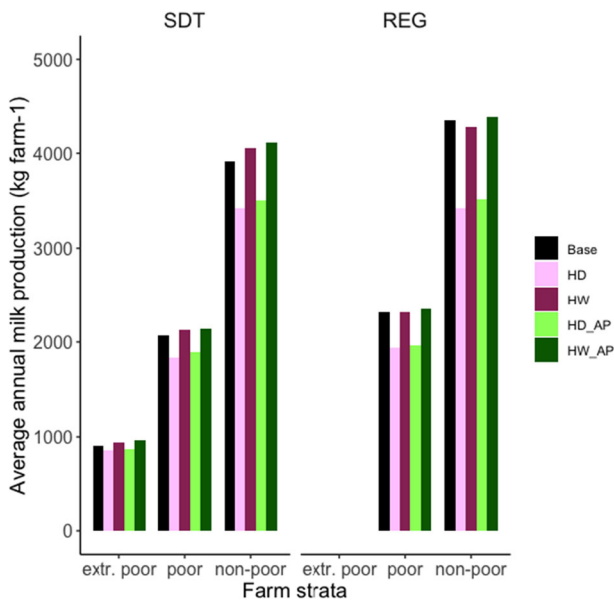
Fig. 7 Impacts of climate change and adaptation (AP) on milk production in cattle-owning farm types (extremely poor (with cattle only in the SDT RAP), poor, and non-poor), as simulated by LIVSIM using APSIM results as input for two contrasting RAPs (SDT sustainable development, REG rapid economic growth). Milk production with no climate change (Base) is compared with milk production under climate change for RCP 4.5 in SDT and 8.5 in REG, each for a hot-dry (HD) and a hot-wet (HW) climate scenario, and with milk production obtained with an adaptation package (AP)
