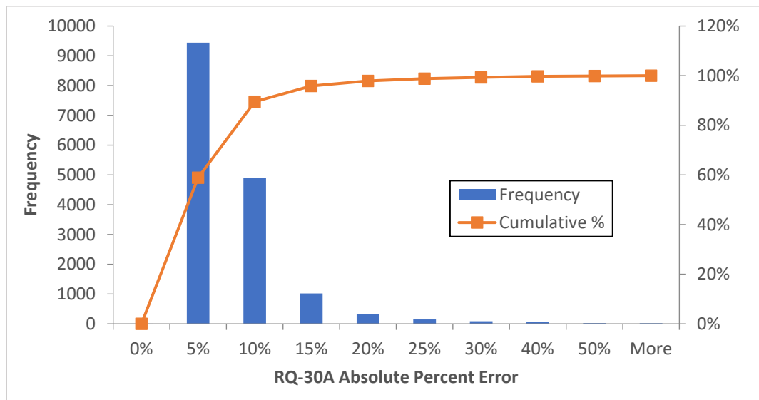
Figure 6. Histogram chart comparing the absolute percent error of the Sommer RQ-30A to the SonTek ADFM
