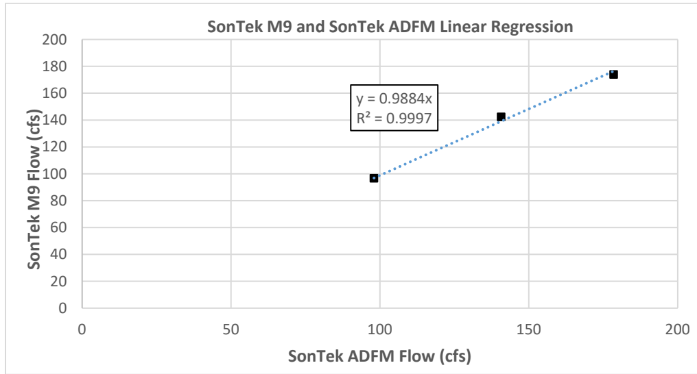
Figure 4. Chart showing SonTek M9 and SonTek ADFM data with regression equation and trendline
