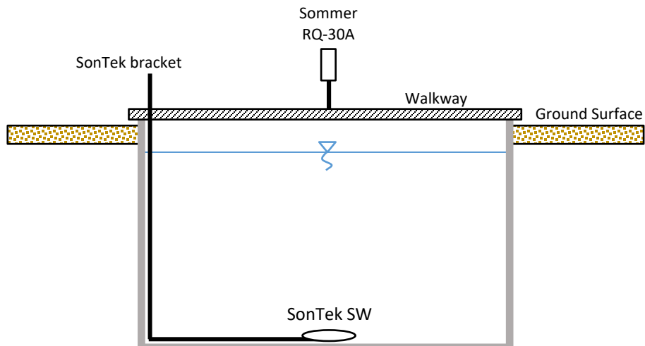
Figure 3. Cross-section view of the subcritical contraction structure showing the positions of the measurement devices, looking downstream
