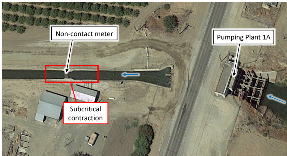
Figure 2. Aerial map view of BCID Main Canal and non-contact meter installation
