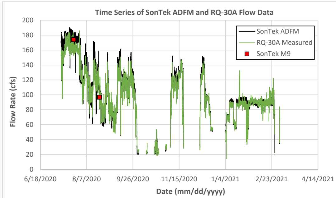
Figure 5. Cumulative data collected at BCID on approximately 15-minute intervals and current metering data (the gaps indicate periods when the flow was below 20 CFS or the sensor(s) did not report flow data).
