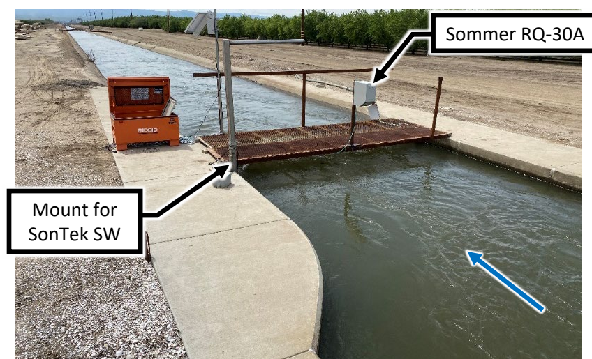
Figure 1. BCID Main Canal subcritical contraction structure with Sommer RQ-30A and SonTek SW
