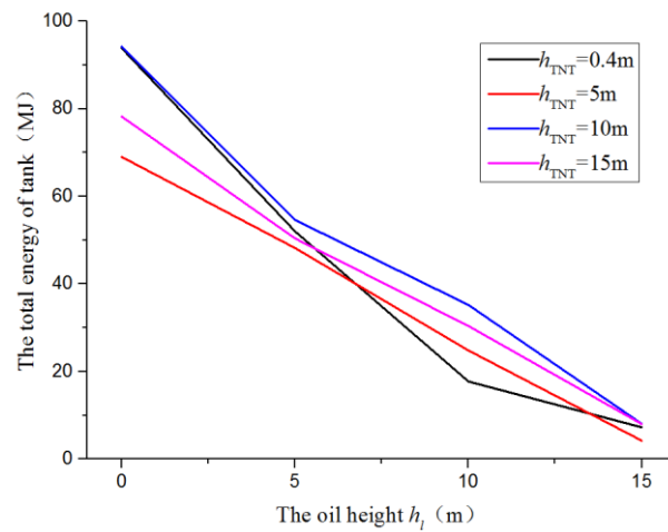
Figure 9. The relationship between the total energy of the fixed-roof storage tank and h_l , h_{TNT} at t=0.08\text{s}
