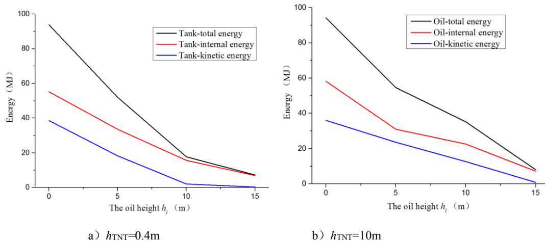
Figure 8. The relationship between the total energy, internal energy, kinetic energy and h_l at t=0.08s
